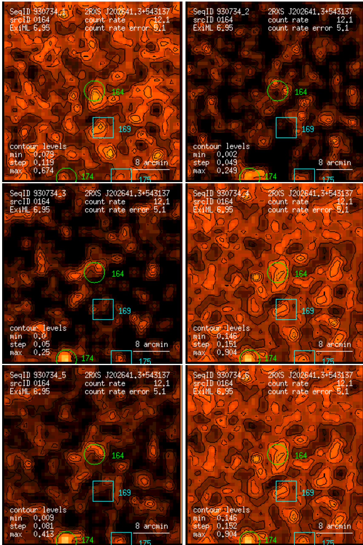
Figure 164: RASS 930734: detection 0164: band rate images, Gaussian filter: (1) PSPC channels 11 – 41, (2) 52 – 90, (3) 91 – 201, (4) 11 – 235, (5) 52 – 201, (6) 11 – 201. Broad band rates in counts/ks. Band rate contour levels in counts/ks/arcmin 2 .
