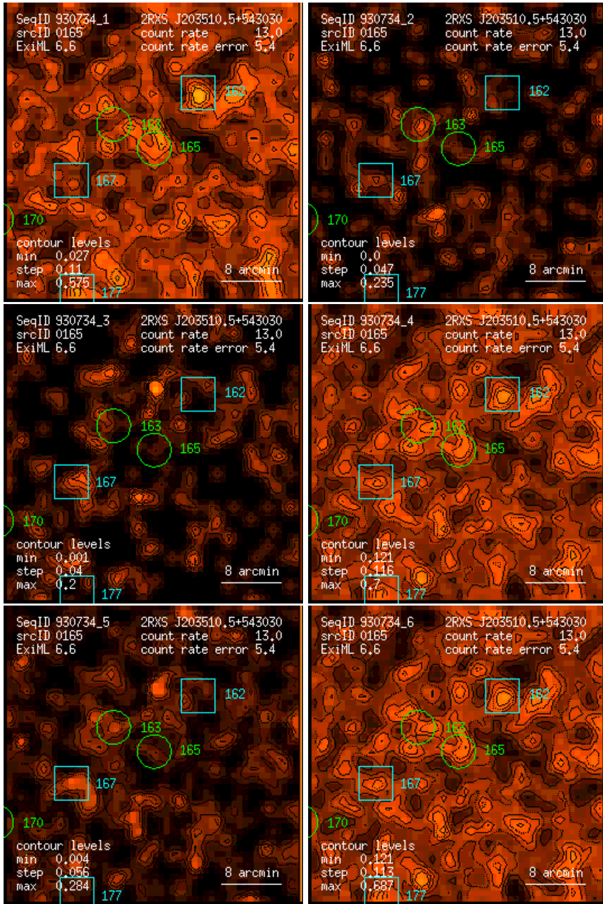
Figure 165: RASS 930734: detection 0165: band rate images, Gaussian filter: (1) PSPC channels 11 – 41, (2) 52 – 90, (3) 91 – 201, (4) 11 – 235, (5) 52 – 201, (6) 11 – 201. Broad band rates in counts/ks. Band rate contour levels in counts/ks/arcmin 2 .
