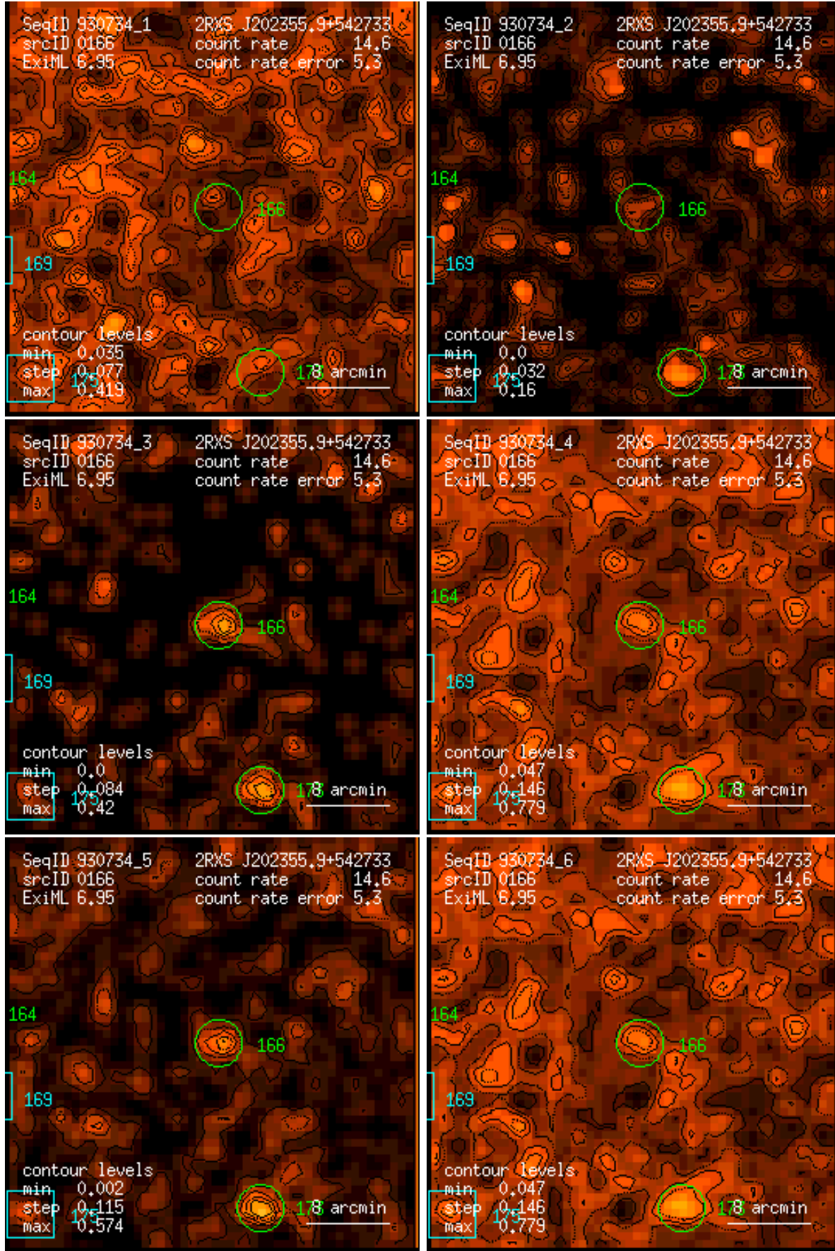
Figure 166: RASS 930734: detection 0166: band rate images, Gaussian filter: (1) PSPC channels 11 – 41, (2) 52 – 90, (3) 91 – 201, (4) 11 – 235, (5) 52 – 201, (6) 11 – 201. Broad band rates in counts/ks. Band rate contour levels in counts/ks/arcmin 2 .
