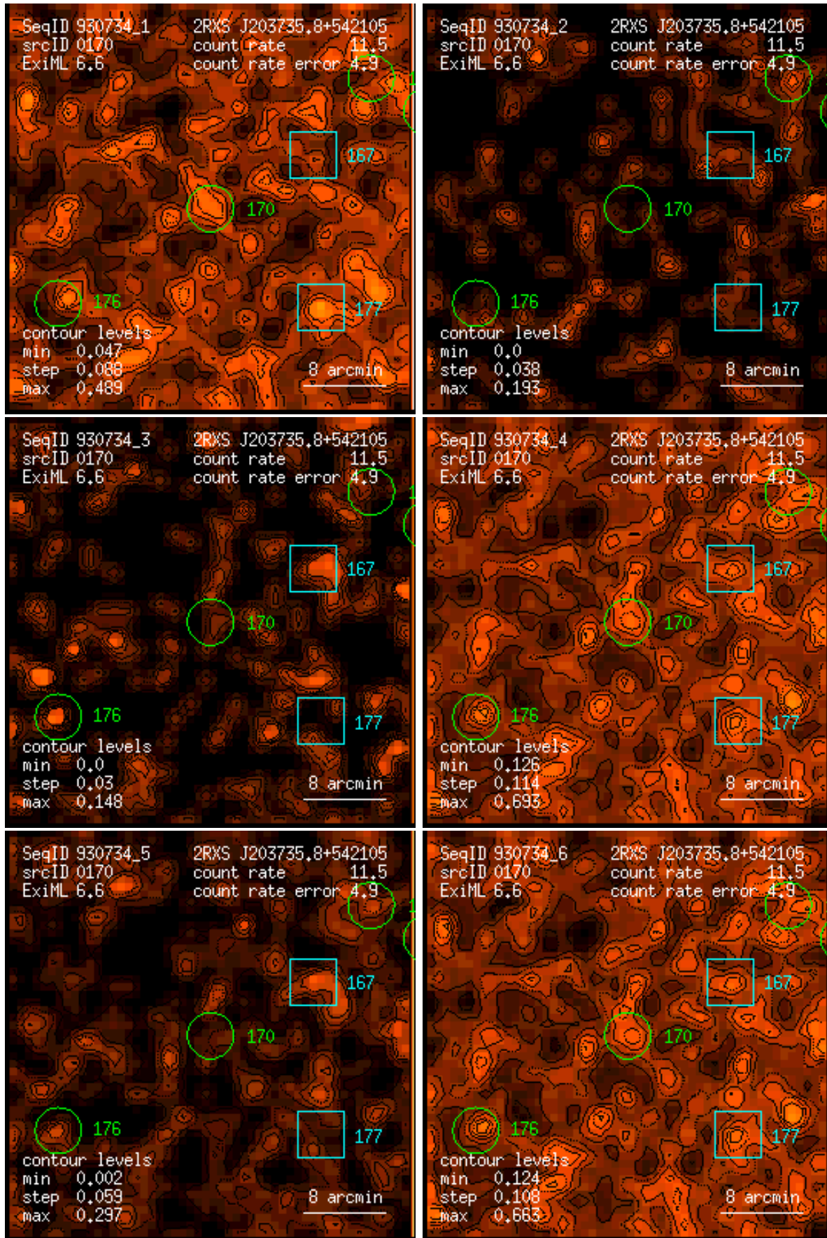
Figure 170: RASS 930734: detection 0170: band rate images, Gaussian filter: (1) PSPC channels 11 – 41, (2) 52 – 90, (3) 91 – 201, (4) 11 – 235, (5) 52 – 201, (6) 11 – 201. Broad band rates in counts/ks. Band rate contour levels in counts/ks/arcmin 2 .
