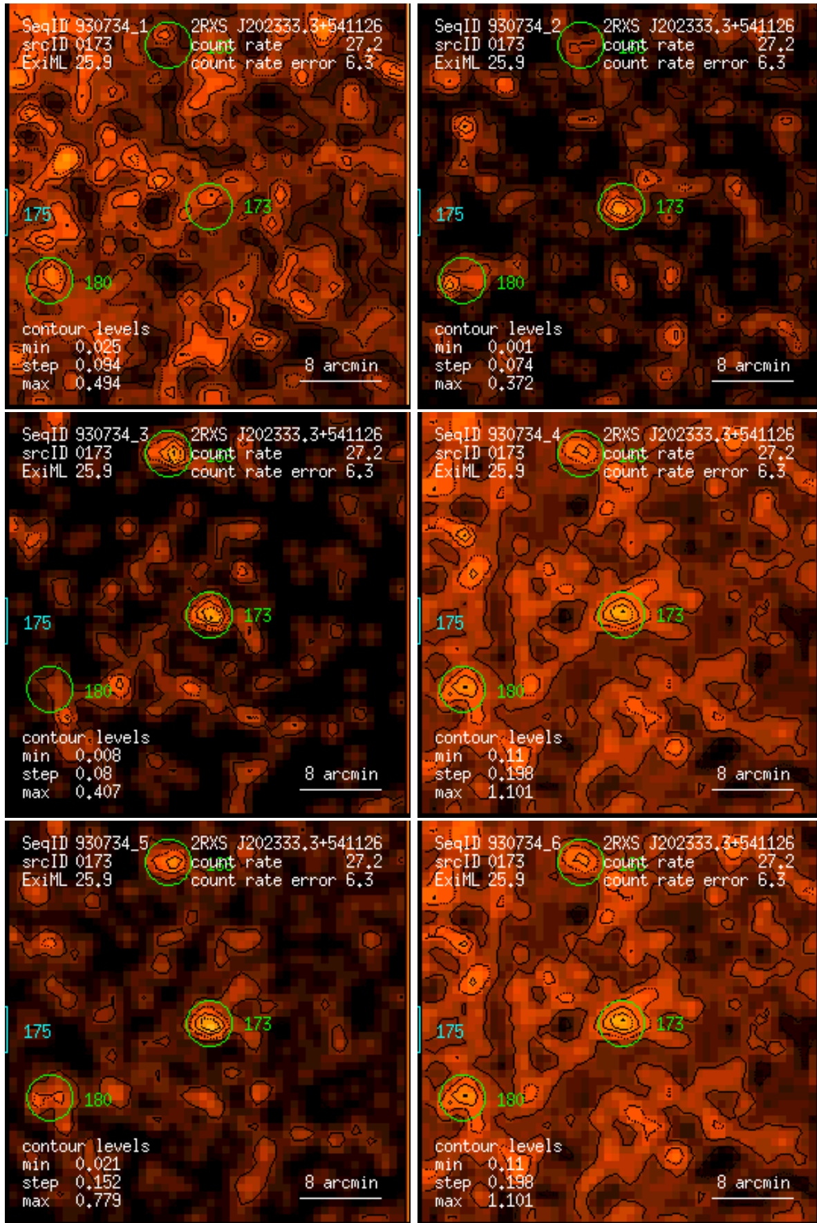
Figure 173: RASS 930734: detection 0173: band rate images, Gaussian filter: (1) PSPC channels 11 – 41, (2) 52 – 90, (3) 91 – 201, (4) 11 – 235, (5) 52 – 201, (6) 11 – 201. Broad band rates in counts/ks. Band rate contour levels in counts/ks/arcmin 2 .
