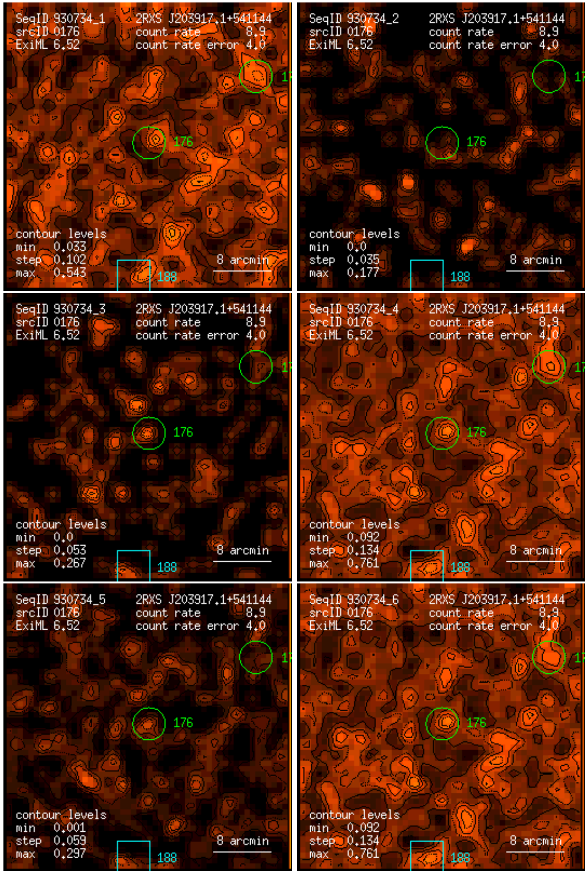
Figure 176: RASS 930734: detection 0176: band rate images, Gaussian filter: (1) PSPC channels 11 – 41, (2) 52 – 90, (3) 91 – 201, (4) 11 – 235, (5) 52 – 201, (6) 11 – 201. Broad band rates in counts/ks. Band rate contour levels in counts/ks/arcmin 2 .
