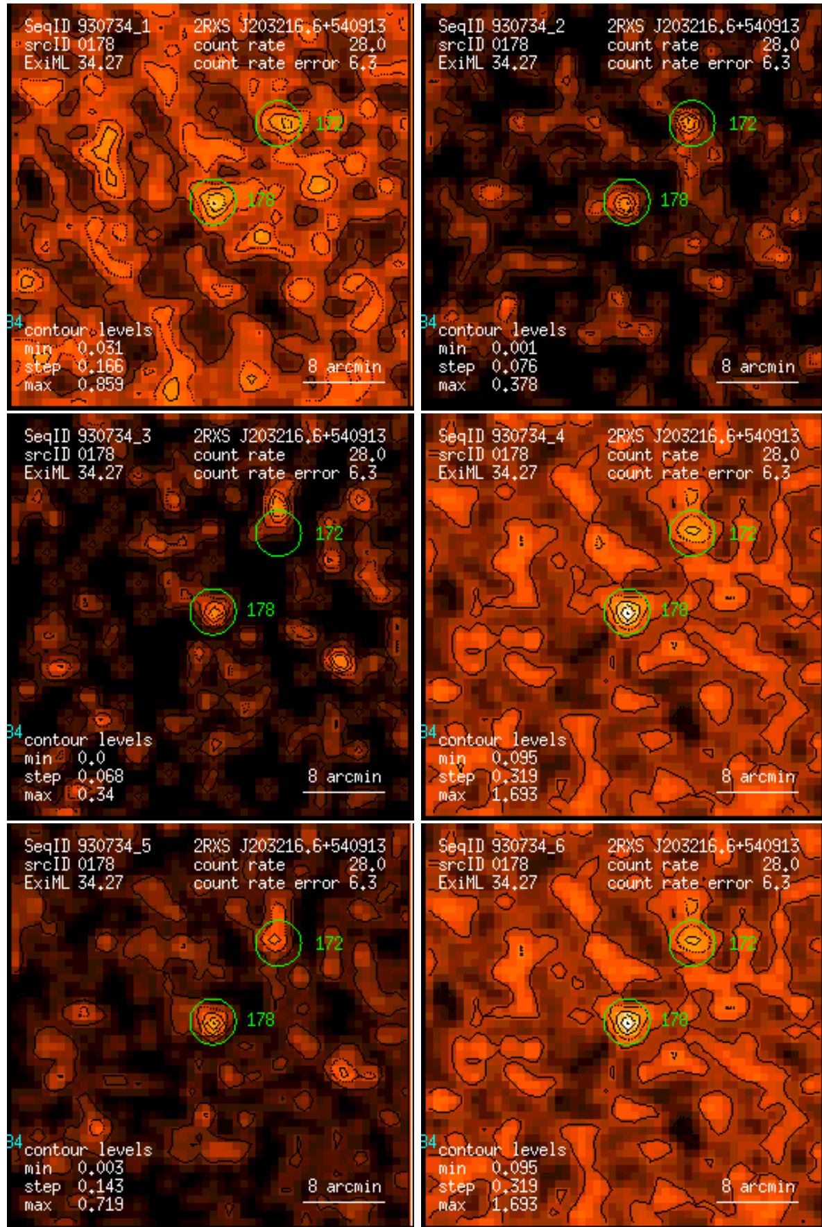
Figure 178: RASS 930734: detection 0178: band rate images, Gaussian filter: (1) PSPC channels 11 – 41, (2) 52 – 90, (3) 91 – 201, (4) 11 – 235, (5) 52 – 201, (6) 11 – 201. Broad band rates in counts/ks. Band rate contour levels in counts/ks/arcmin 2 .
