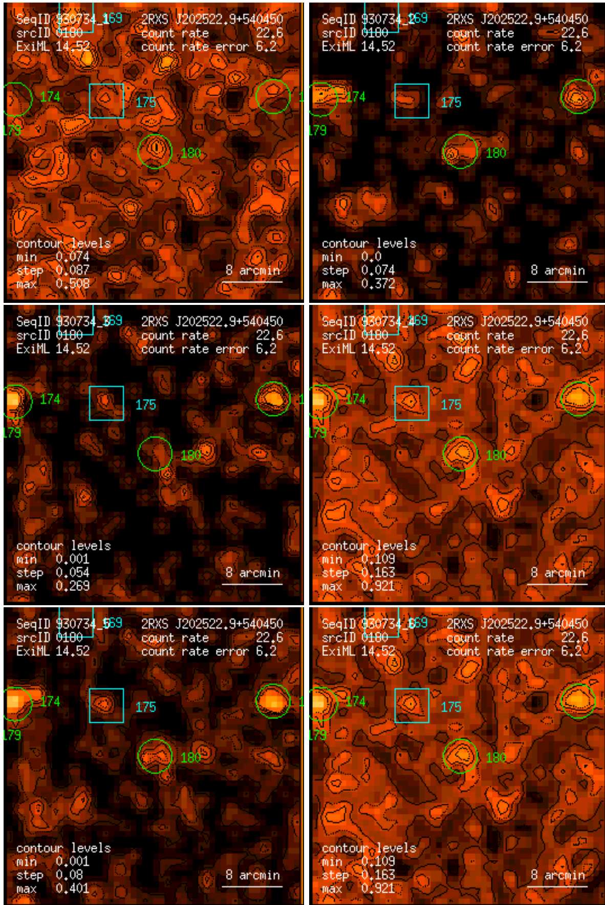
Figure 180: RASS 930734: detection 0180: band rate images, Gaussian filter: (1) PSPC channels 11 – 41, (2) 52 – 90, (3) 91 – 201, (4) 11 – 235, (5) 52 – 201, (6) 11 – 201. Broad band rates in counts/ks. Band rate contour levels in counts/ks/arcmin 2 .
