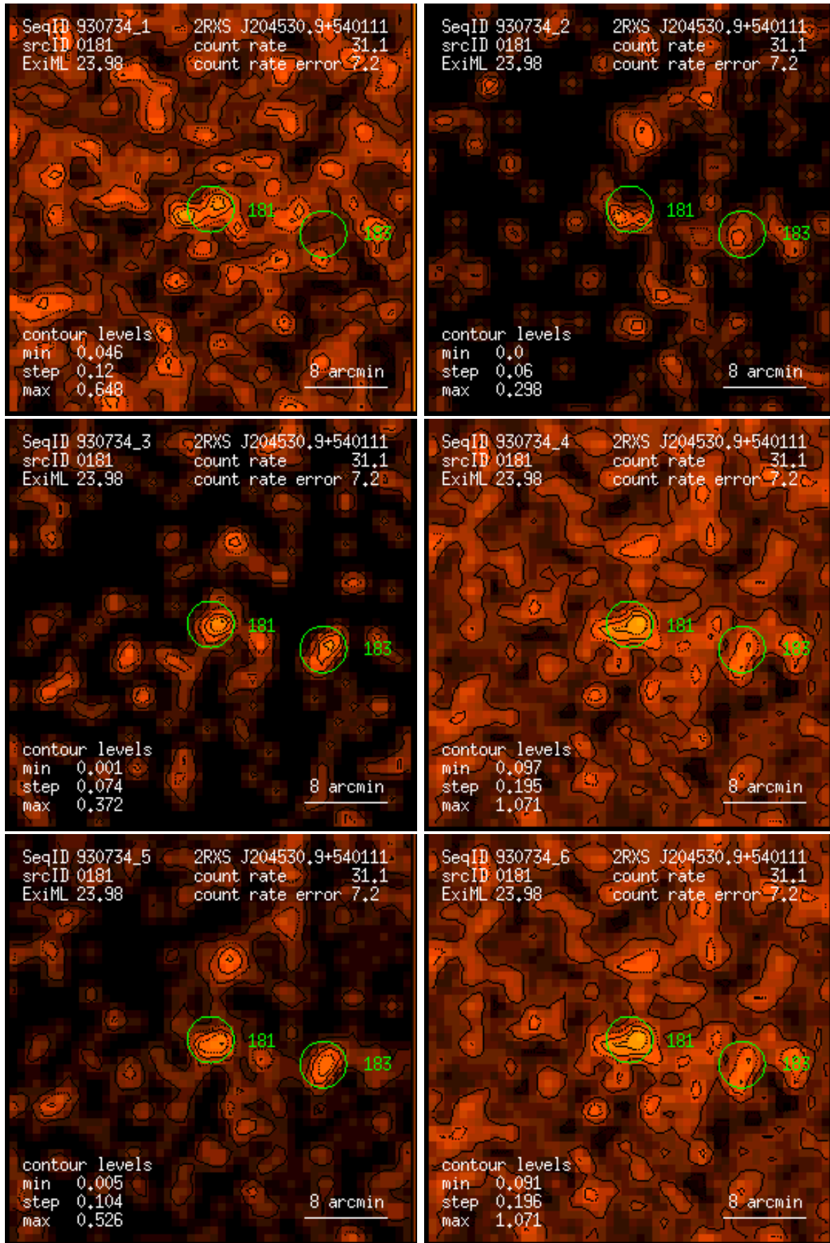
Figure 181: RASS 930734: detection 0181: band rate images, Gaussian filter: (1) PSPC channels 11 – 41, (2) 52 – 90, (3) 91 – 201, (4) 11 – 235, (5) 52 – 201, (6) 11 – 201. Broad band rates in counts/ks. Band rate contour levels in counts/ks/arcmin 2 .
