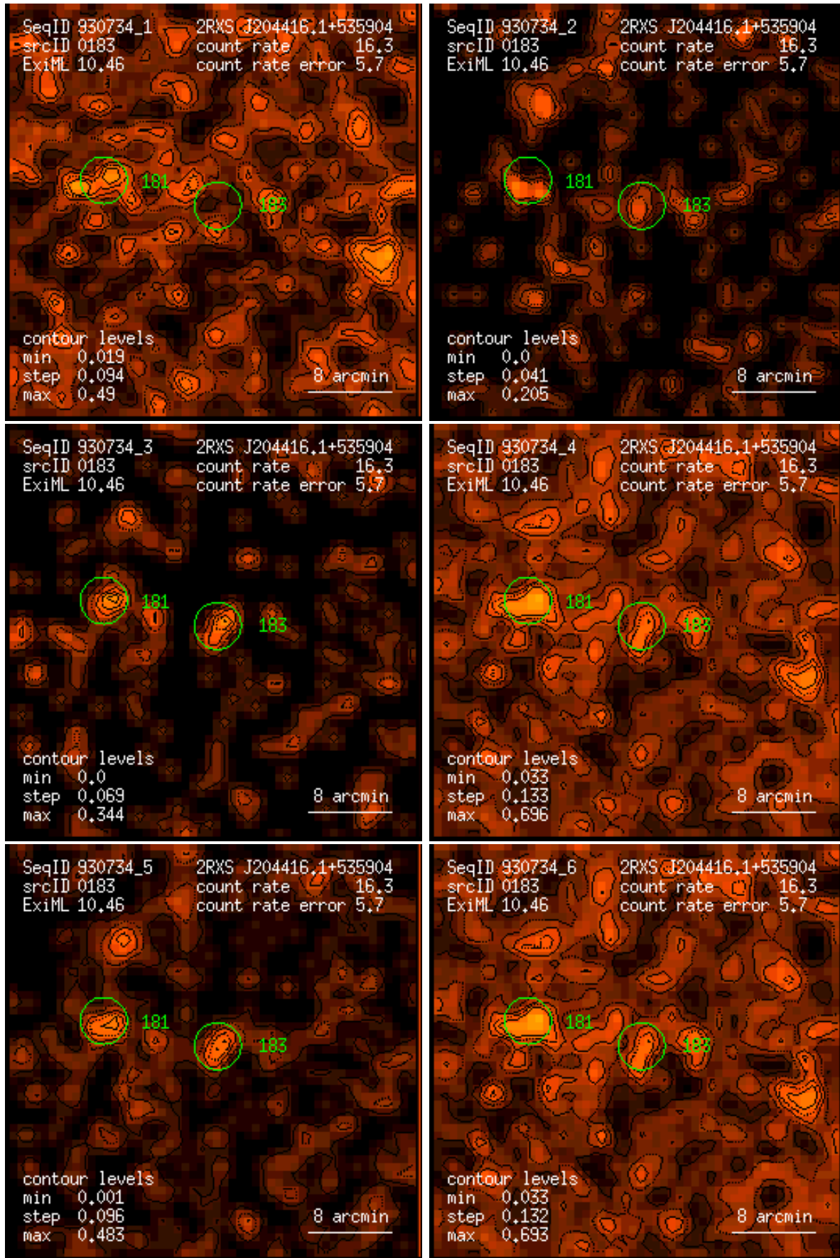
Figure 183: RASS 930734: detection 0183: band rate images, Gaussian filter: (1) PSPC channels 11 – 41, (2) 52 – 90, (3) 91 – 201, (4) 11 – 235, (5) 52 – 201, (6) 11 – 201. Broad band rates in counts/ks. Band rate contour levels in counts/ks/arcmin 2 .
