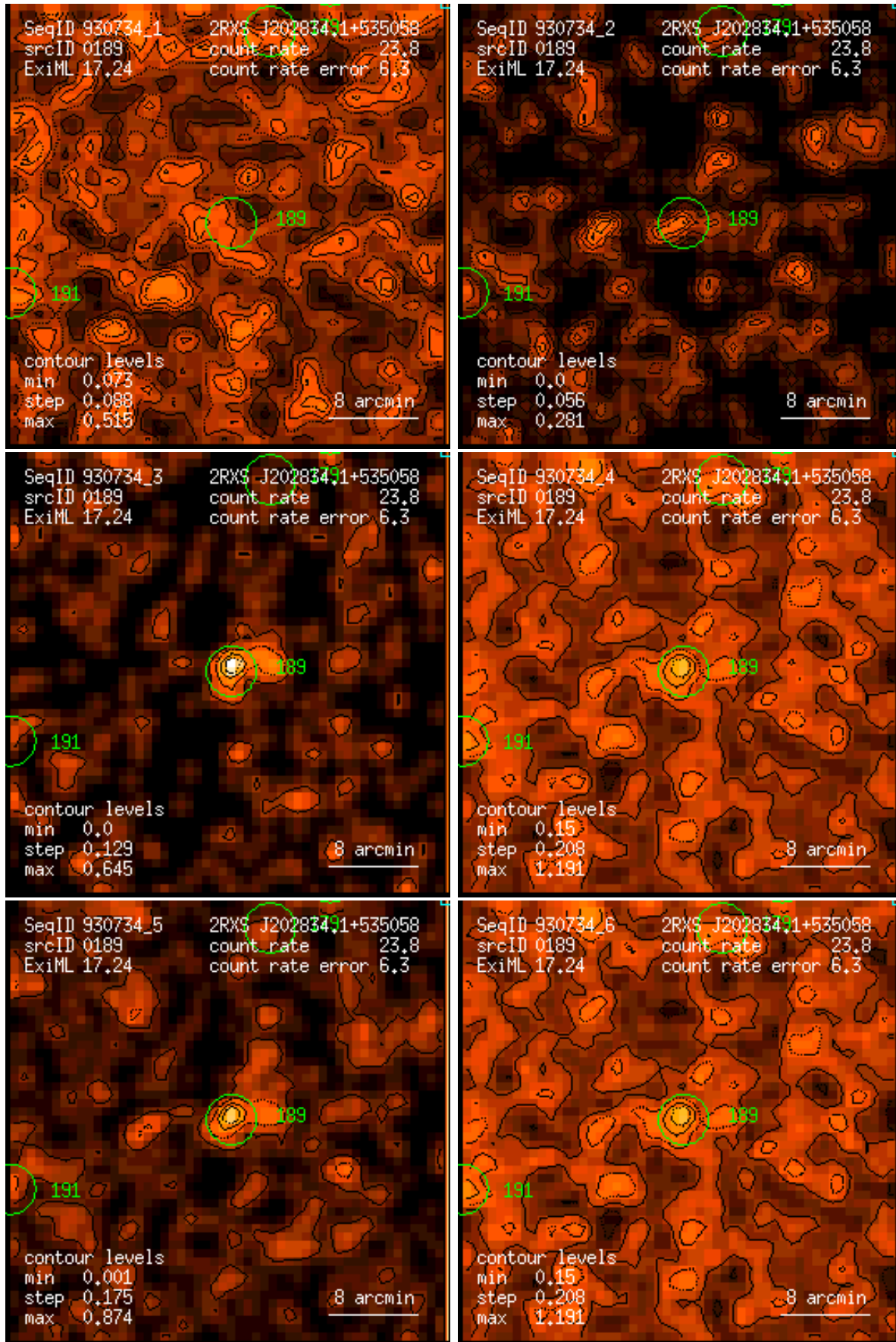
Figure 189: RASS 930734: detection 0189: band rate images, Gaussian filter: (1) PSPC channels 11 – 41, (2) 52 – 90, (3) 91 – 201, (4) 11 – 235, (5) 52 – 201, (6) 11 – 201. Broad band rates in counts/ks. Band rate contour levels in counts/ks/arcmin 2 .
