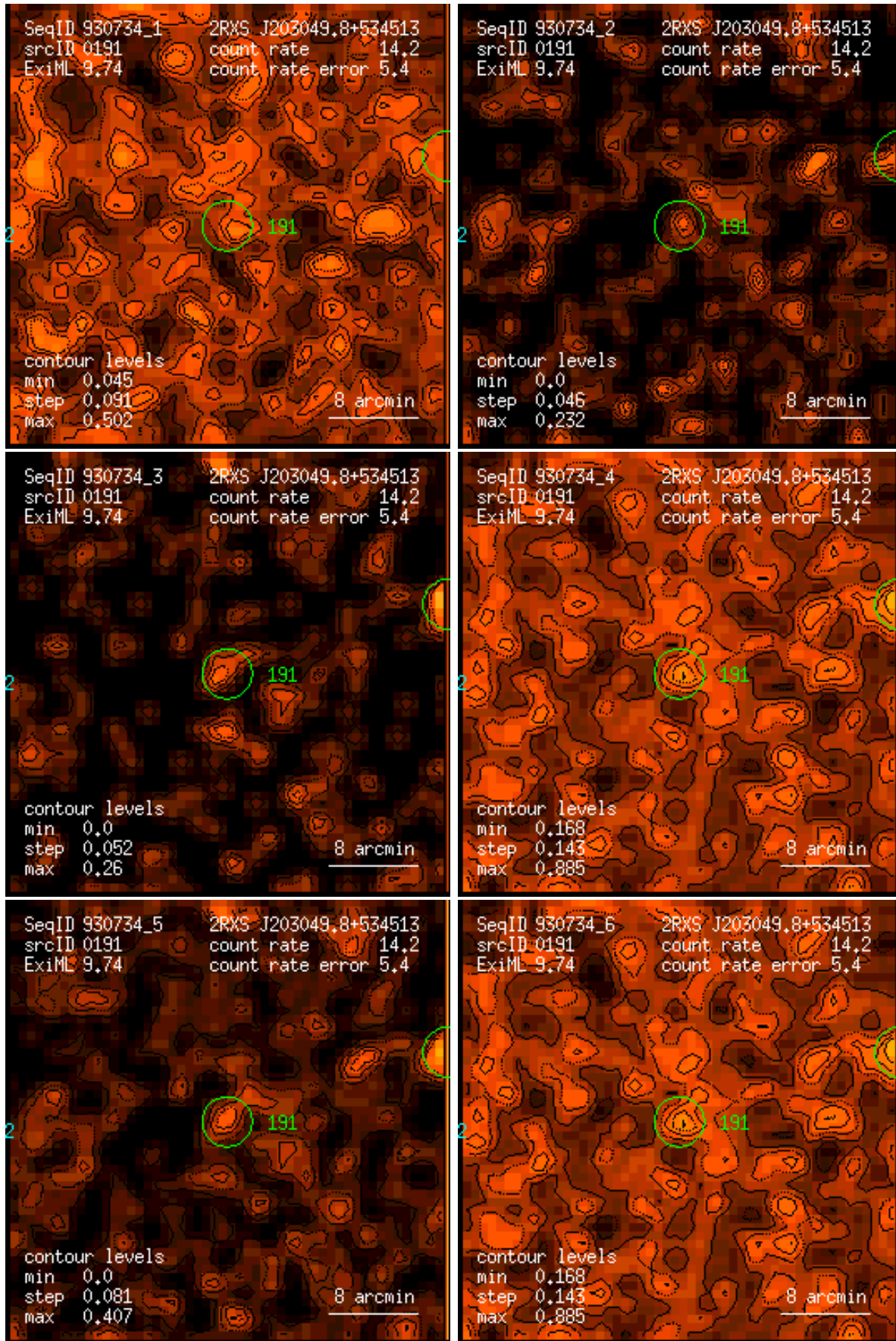
Figure 191: RASS 930734: detection 0191: band rate images, Gaussian filter: (1) PSPC channels 11 – 41, (2) 52 – 90, (3) 91 – 201, (4) 11 – 235, (5) 52 – 201, (6) 11 – 201. Broad band rates in counts/ks. Band rate contour levels in counts/ks/arcmin 2 .
