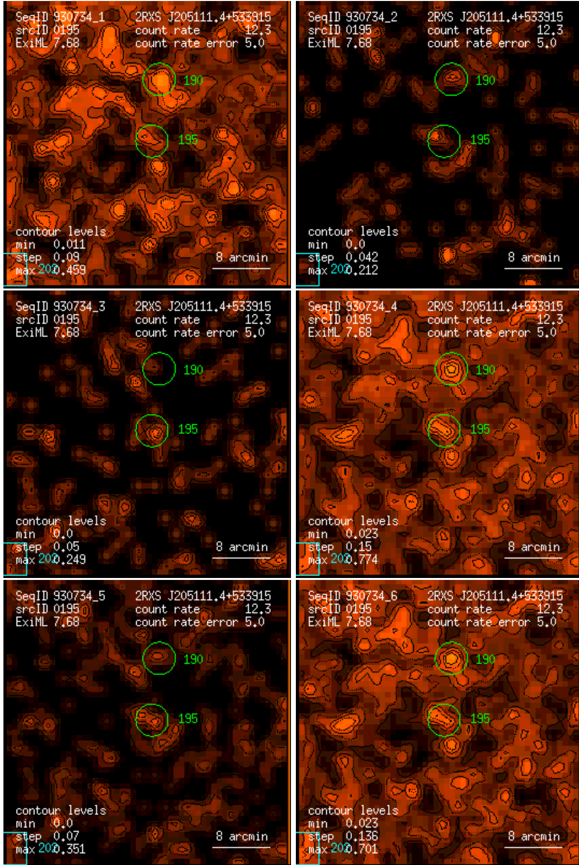
Figure 195: RASS 930734: detection 0195: band rate images, Gaussian filter: (1) PSPC channels 11 – 41, (2) 52 – 90, (3) 91 – 201, (4) 11 – 235, (5) 52 – 201, (6) 11 – 201. Broad band rates in counts/ks. Band rate contour levels in counts/ks/arcmin 2 .
