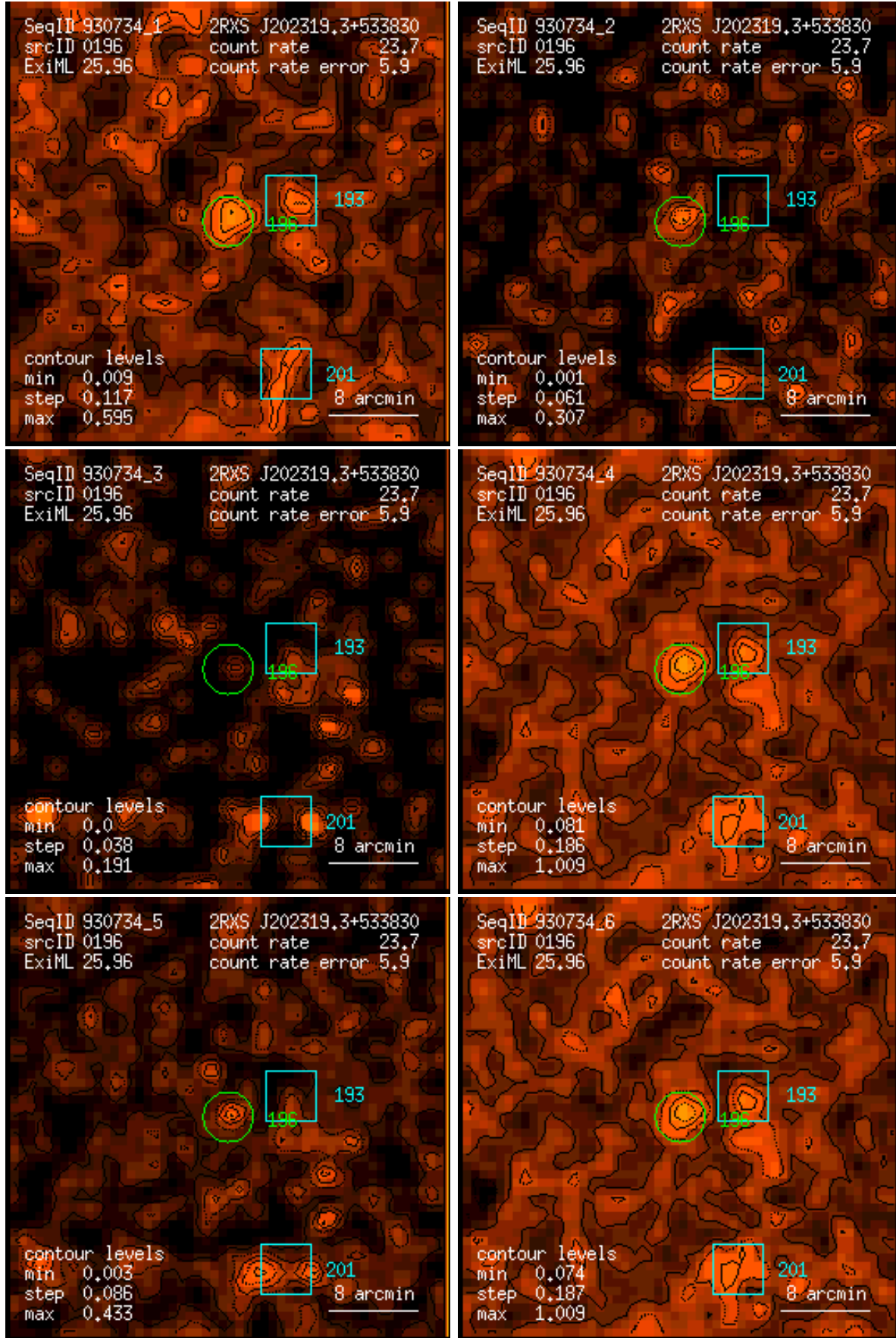
Figure 196: RASS 930734: detection 0196: band rate images, Gaussian filter: (1) PSPC channels 11 – 41, (2) 52 – 90, (3) 91 – 201, (4) 11 – 235, (5) 52 – 201, (6) 11 – 201. Broad band rates in counts/ks. Band rate contour levels in counts/ks/arcmin 2 .
