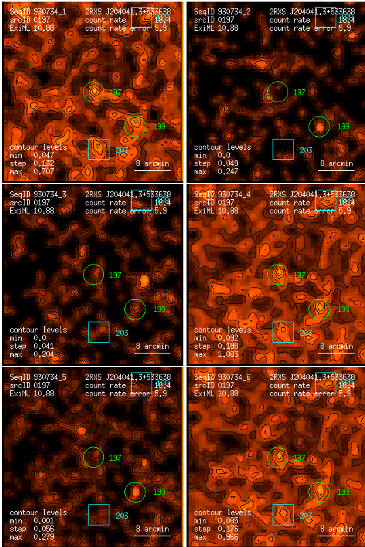
Figure 197: RASS 930734: detection 0197: band rate images, Gaussian filter: (1) PSPC channels 11 – 41, (2) 52 – 90, (3) 91 – 201, (4) 11 – 235, (5) 52 – 201, (6) 11 – 201. Broad band rates in counts/ks. Band rate contour levels in counts/ks/arcmin 2 .
