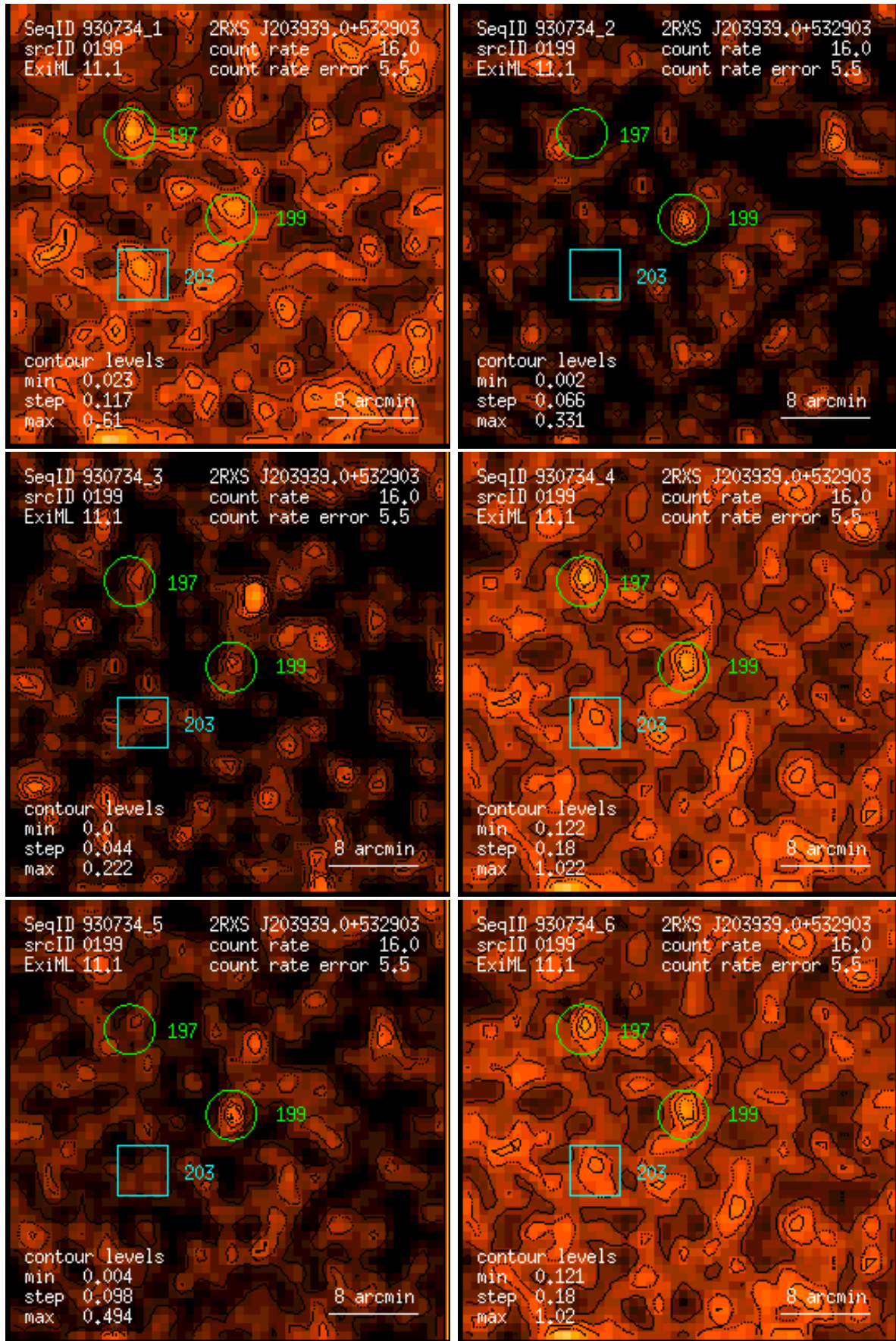
Figure 199: RASS 930734: detection 0199: band rate images, Gaussian filter: (1) PSPC channels 11 – 41, (2) 52 – 90, (3) 91 – 201, (4) 11 – 235, (5) 52 – 201, (6) 11 – 201. Broad band rates in counts/ks. Band rate contour levels in counts/ks/arcmin 2 .
