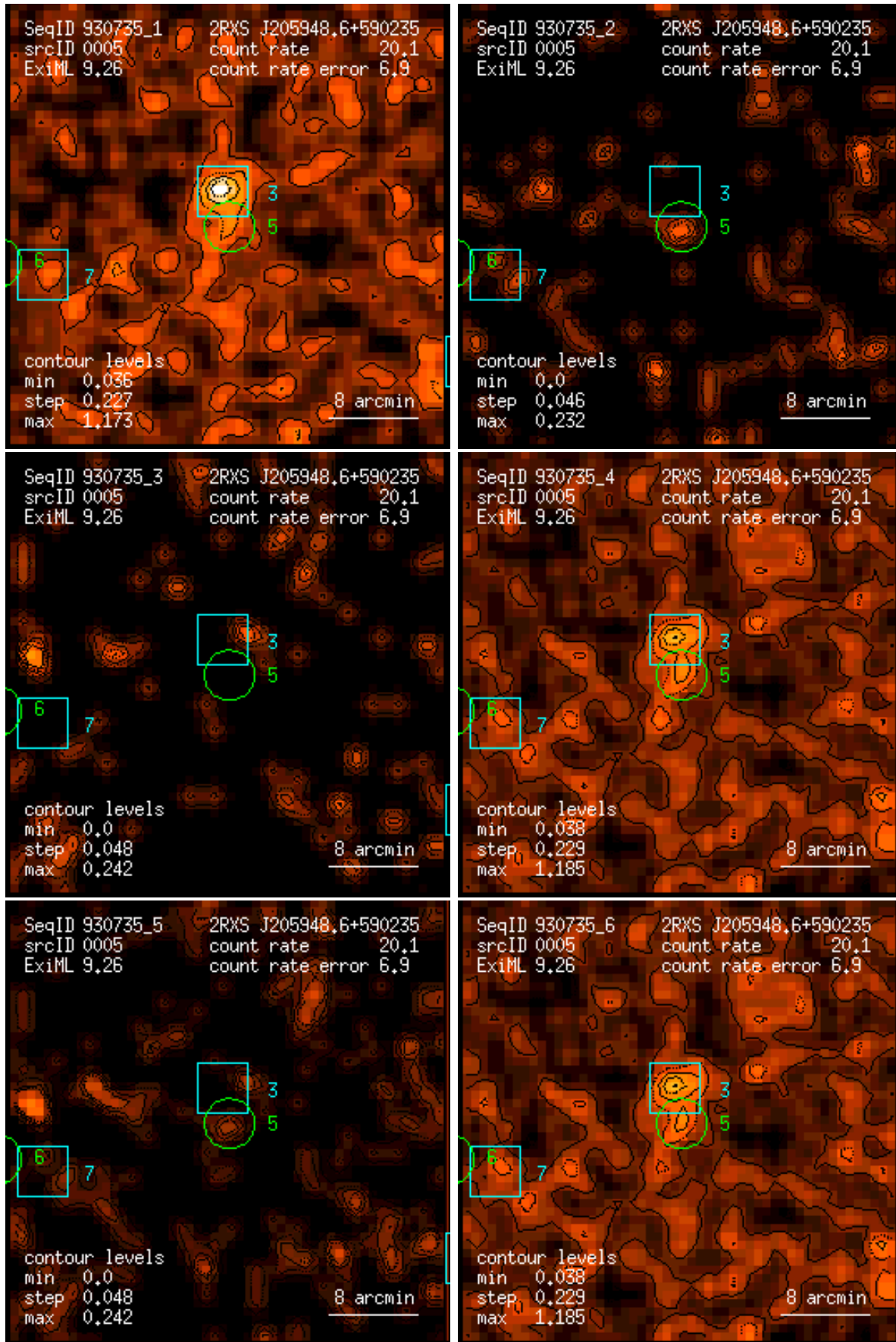
Figure 5: RASS 930735: detection 0005: band rate images, Gaussian filter: (1) PSPC channels 11 – 41, (2) 52 – 90, (3) 91 – 201, (4) 11 – 235, (5) 52 – 201, (6) 11 – 201. Broad band rates in counts/ks. Band rate contour levels in counts/ks/arcmin 2 .
