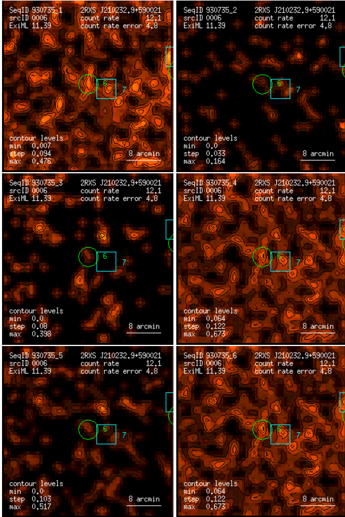
Figure 6: RASS 930735: detection 0006: band rate images, Gaussian filter: (1) PSPC channels 11 – 41, (2) 52 – 90, (3) 91 – 201, (4) 11 – 235, (5) 52 – 201, (6) 11 – 201. Broad band rates in counts/ks. Band rate contour levels in counts/ks/arcmin 2 .
