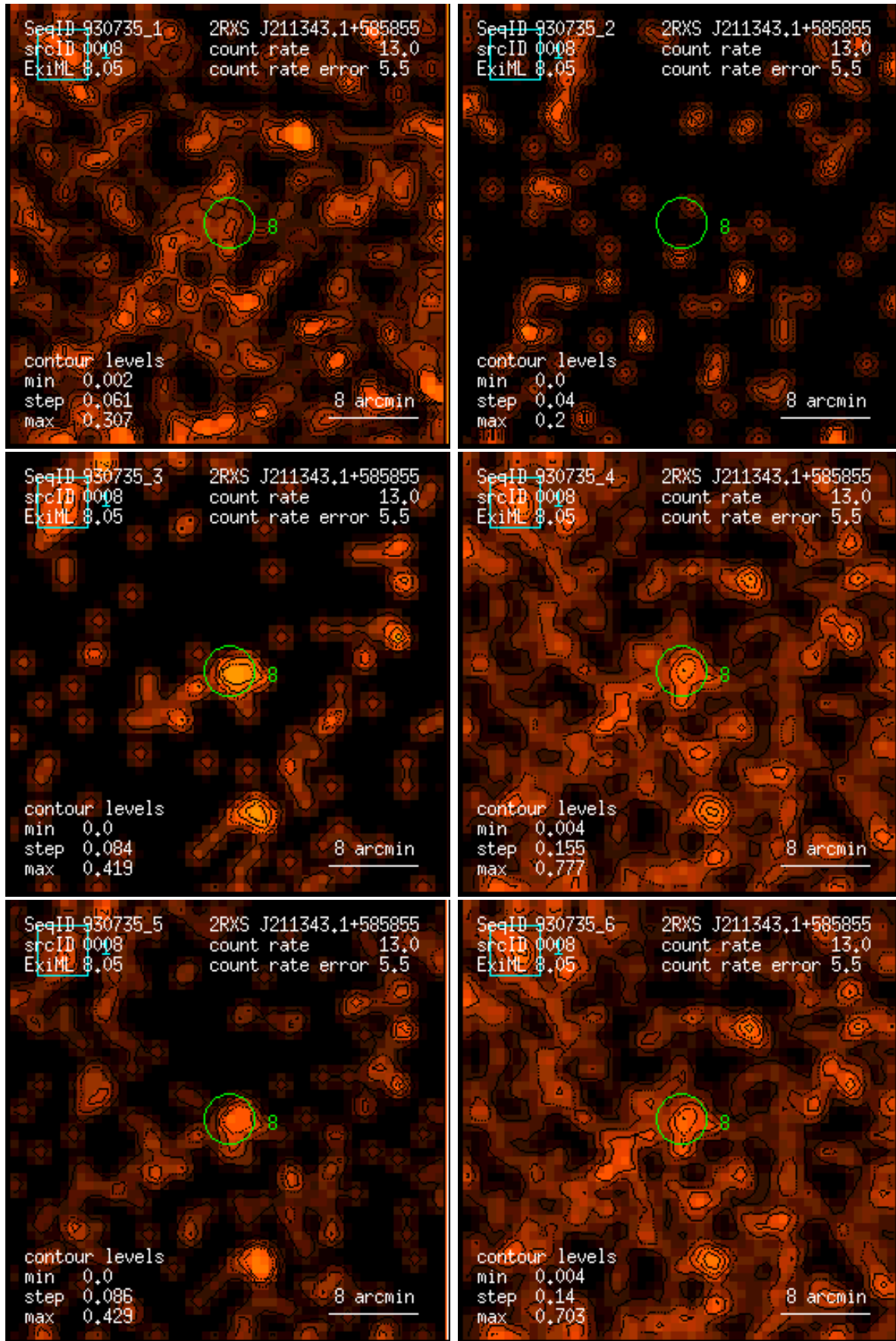
Figure 8: RASS 930735: detection 0008: band rate images, Gaussian filter: (1) PSPC channels 11 – 41, (2) 52 – 90, (3) 91 – 201, (4) 11 – 235, (5) 52 – 201, (6) 11 – 201. Broad band rates in counts/ks. Band rate contour levels in counts/ks/arcmin 2 .
