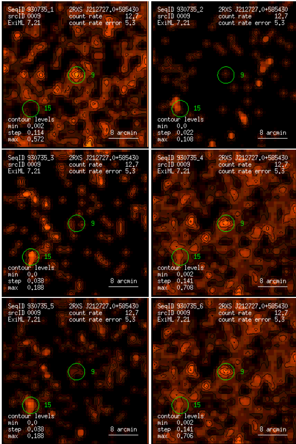
Figure 9: RASS 930735: detection 0009: band rate images, Gaussian filter: (1) PSPC channels 11 – 41, (2) 52 – 90, (3) 91 – 201, (4) 11 – 235, (5) 52 – 201, (6) 11 – 201. Broad band rates in counts/ks. Band rate contour levels in counts/ks/arcmin 2 .
