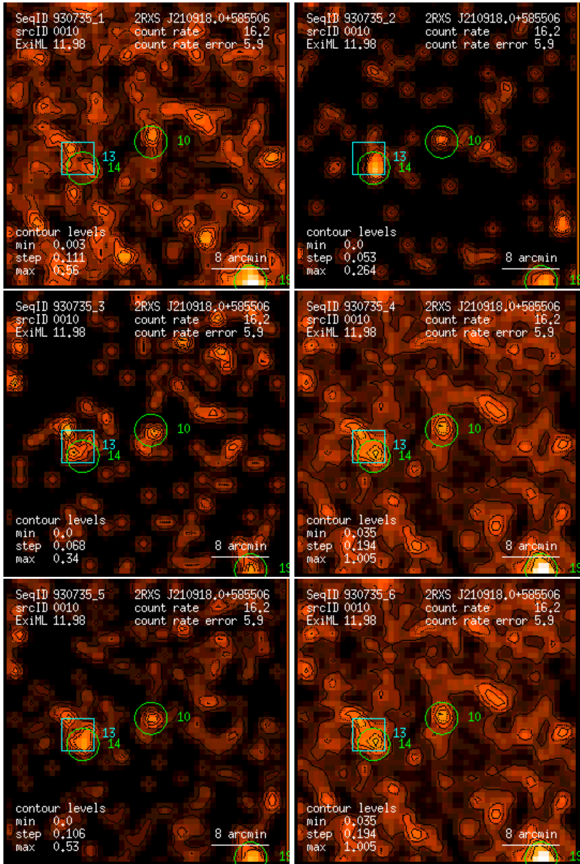
Figure 10: RASS 930735: detection 0010: band rate images, Gaussian filter: (1) PSPC channels 11 – 41, (2) 52 – 90, (3) 91 – 201, (4) 11 – 235, (5) 52 – 201, (6) 11 – 201. Broad band rates in counts/ks. Band rate contour levels in counts/ks/arcmin 2 .
