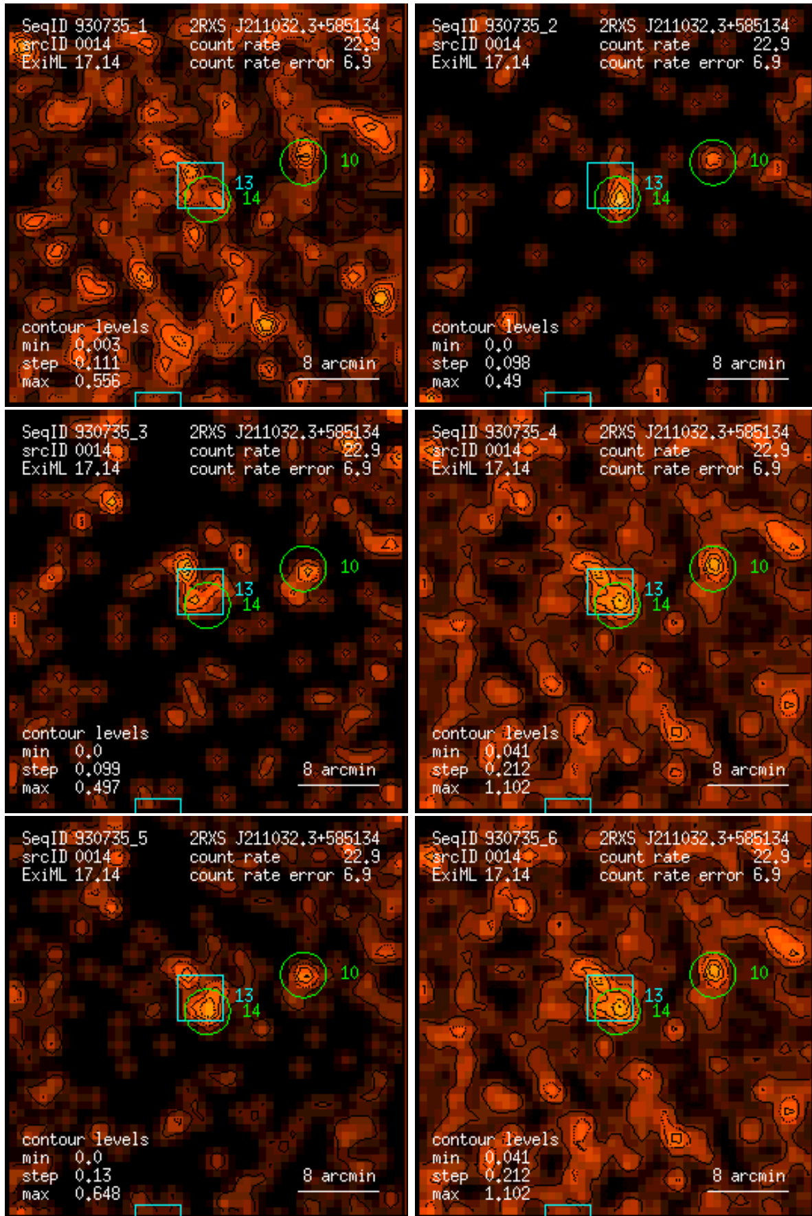
Figure 14: RASS 930735: detection 0014: band rate images, Gaussian filter: (1) PSPC channels 11 – 41, (2) 52 – 90, (3) 91 – 201, (4) 11 – 235, (5) 52 – 201, (6) 11 – 201. Broad band rates in counts/ks. Band rate contour levels in counts/ks/arcmin 2 .
