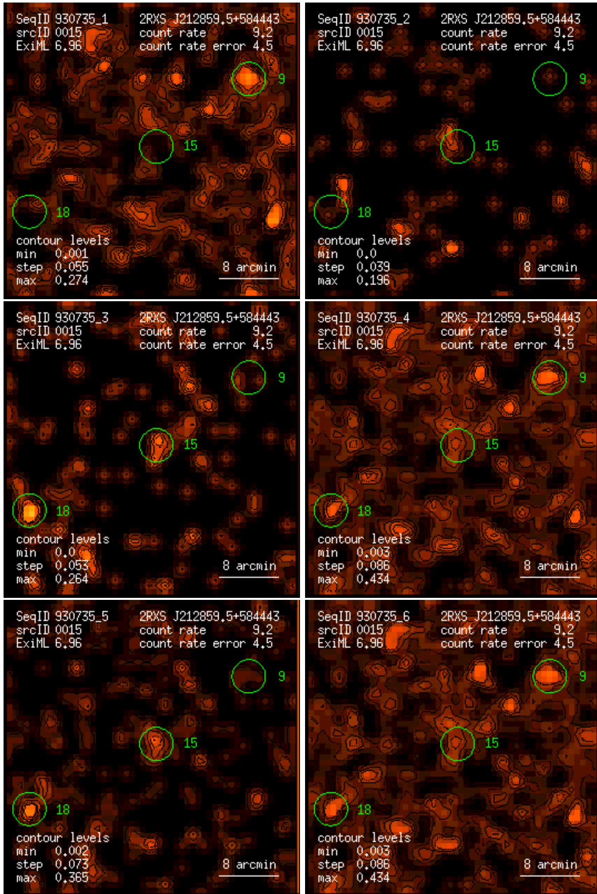
Figure 15: RASS 930735: detection 0015: band rate images, Gaussian filter: (1) PSPC channels 11 – 41, (2) 52 – 90, (3) 91 – 201, (4) 11 – 235, (5) 52 – 201, (6) 11 – 201. Broad band rates in counts/ks. Band rate contour levels in counts/ks/arcmin 2 .
