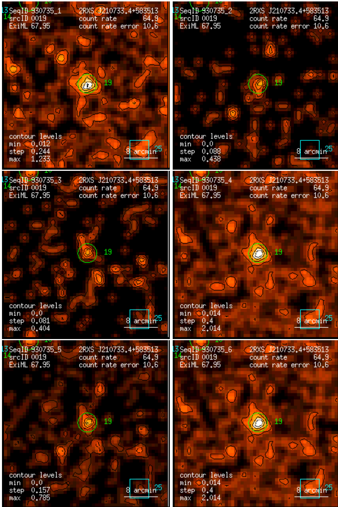
Figure 19: RASS 930735: detection 0019: band rate images, Gaussian filter: (1) PSPC channels 11 – 41, (2) 52 – 90, (3) 91 – 201, (4) 11 – 235, (5) 52 – 201, (6) 11 – 201. Broad band rates in counts/ks. Band rate contour levels in counts/ks/arcmin 2 .
