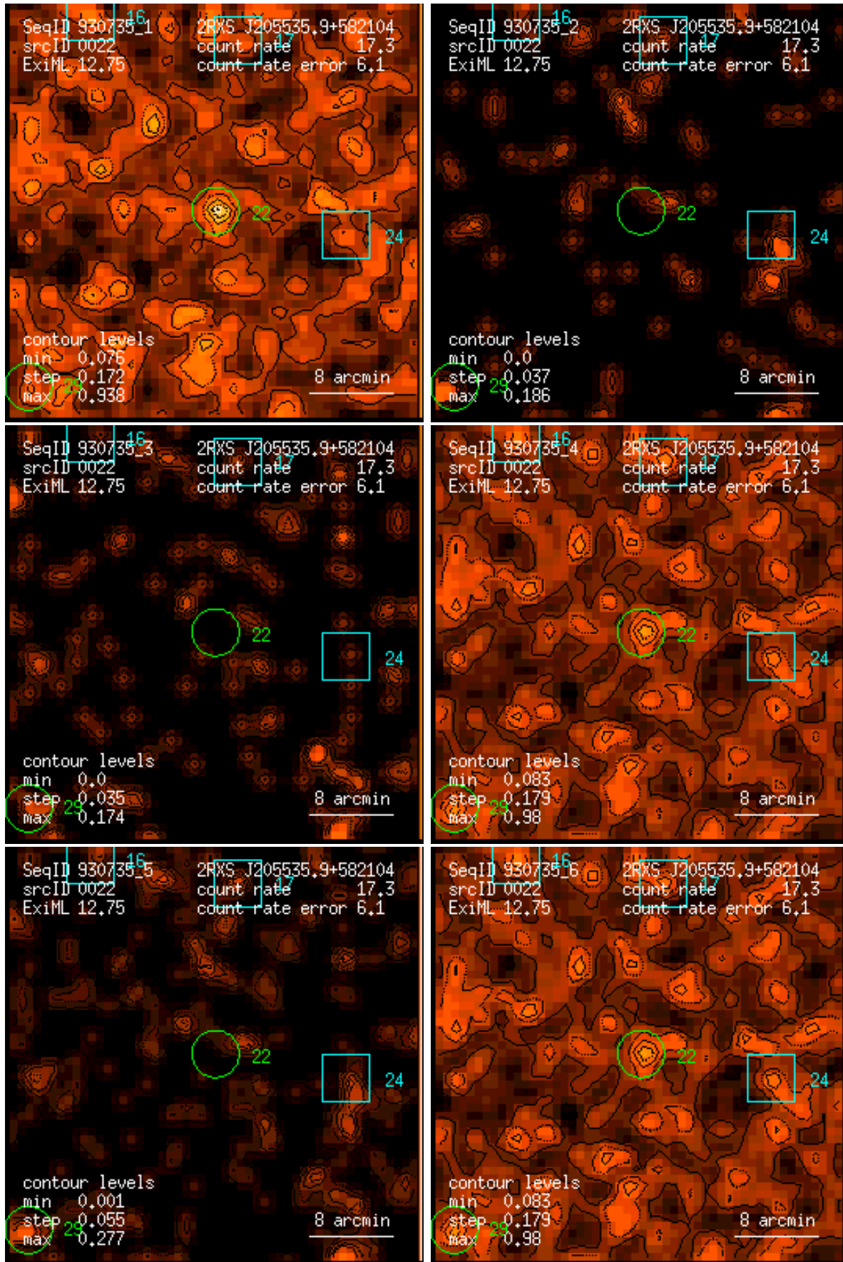
Figure 22: RASS 930735: detection 0022: band rate images, Gaussian filter: (1) PSPC channels 11 – 41, (2) 52 – 90, (3) 91 – 201, (4) 11 – 235, (5) 52 – 201, (6) 11 – 201. Broad band rates in counts/ks. Band rate contour levels in counts/ks/arcmin 2 .
