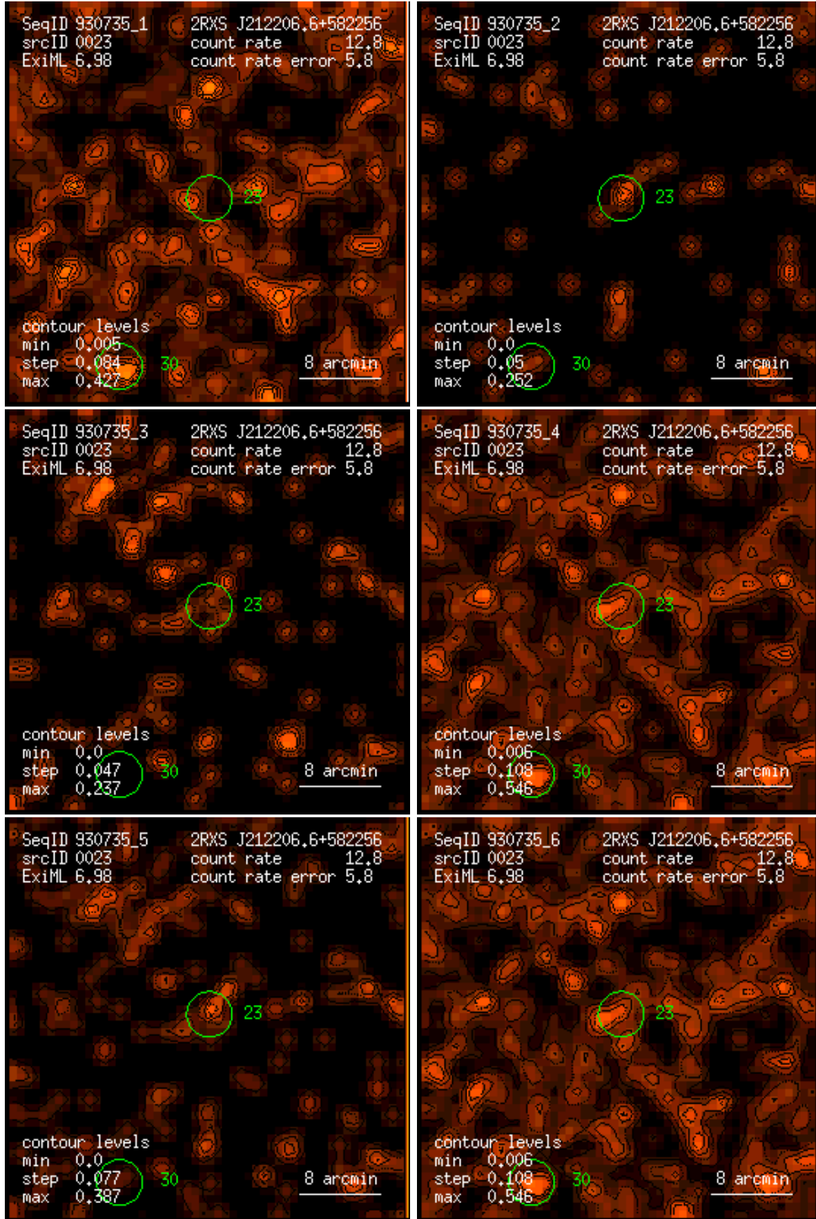
Figure 23: RASS 930735: detection 0023: band rate images, Gaussian filter: (1) PSPC channels 11 – 41, (2) 52 – 90, (3) 91 – 201, (4) 11 – 235, (5) 52 – 201, (6) 11 – 201. Broad band rates in counts/ks. Band rate contour levels in counts/ks/arcmin 2 .
