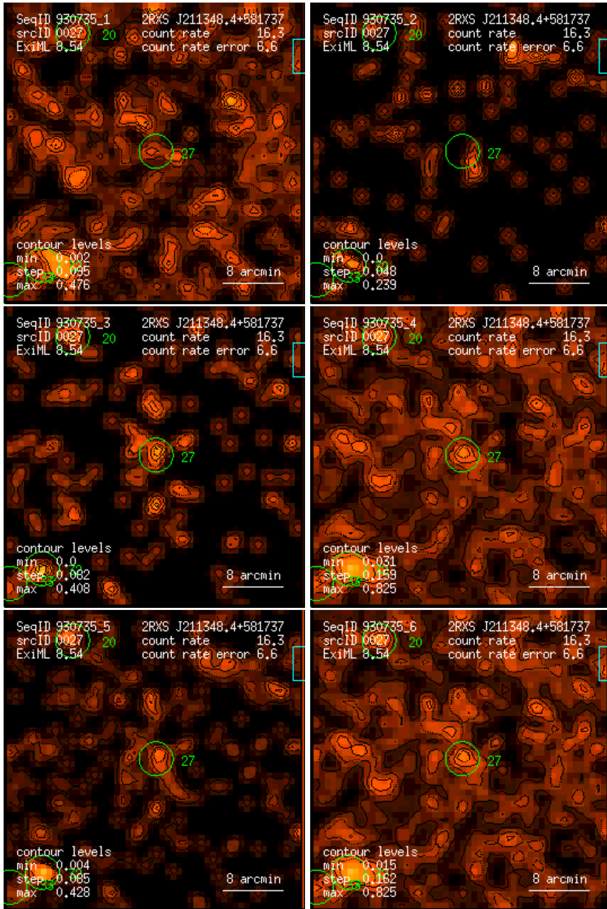
Figure 27: RASS 930735: detection 0027: band rate images, Gaussian filter: (1) PSPC channels 11 – 41, (2) 52 – 90, (3) 91 – 201, (4) 11 – 235, (5) 52 – 201, (6) 11 – 201. Broad band rates in counts/ks. Band rate contour levels in counts/ks/arcmin 2 .
