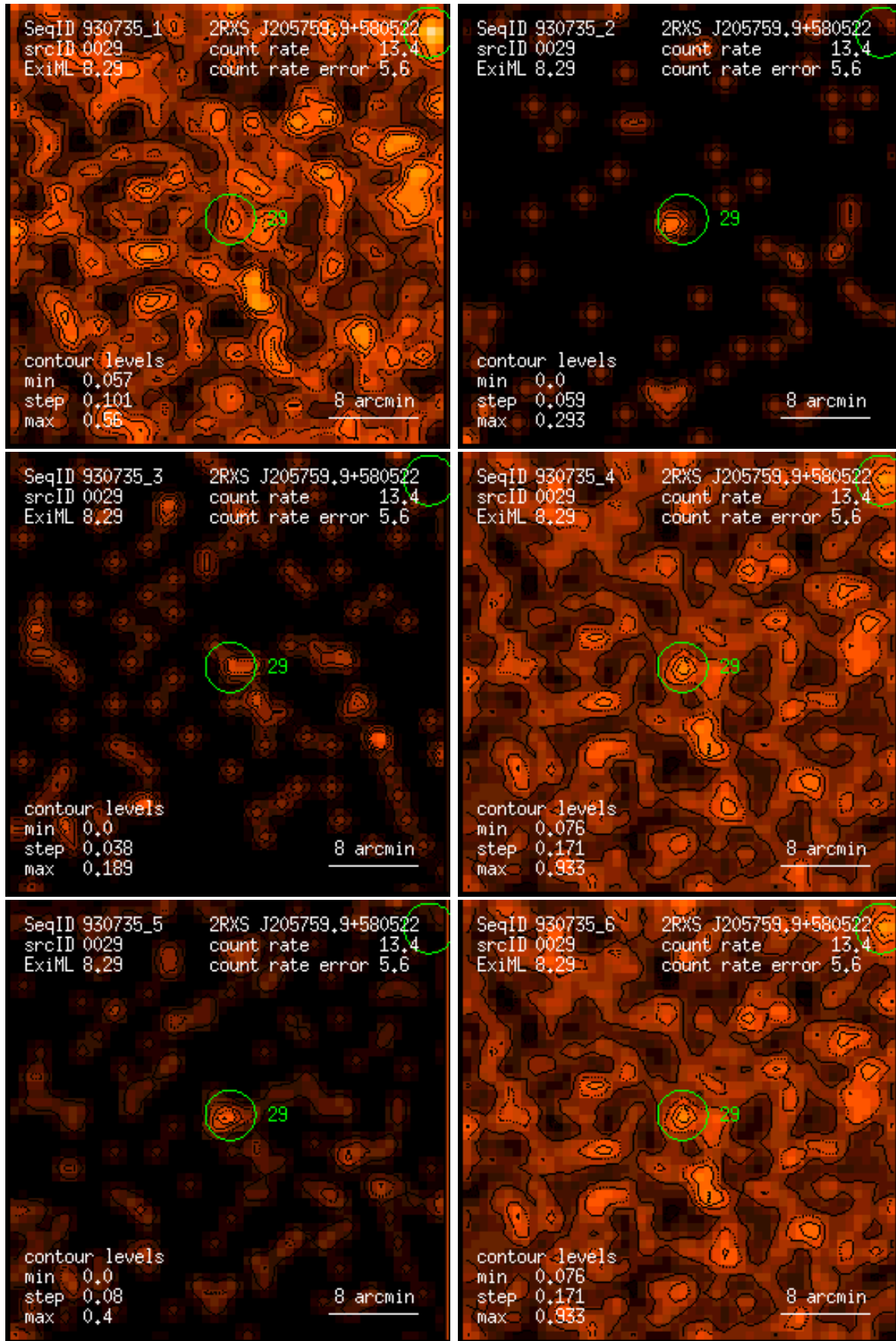
Figure 29: RASS 930735: detection 0029: band rate images, Gaussian filter: (1) PSPC channels 11 – 41, (2) 52 – 90, (3) 91 – 201, (4) 11 – 235, (5) 52 – 201, (6) 11 – 201. Broad band rates in counts/ks. Band rate contour levels in counts/ks/arcmin 2 .
