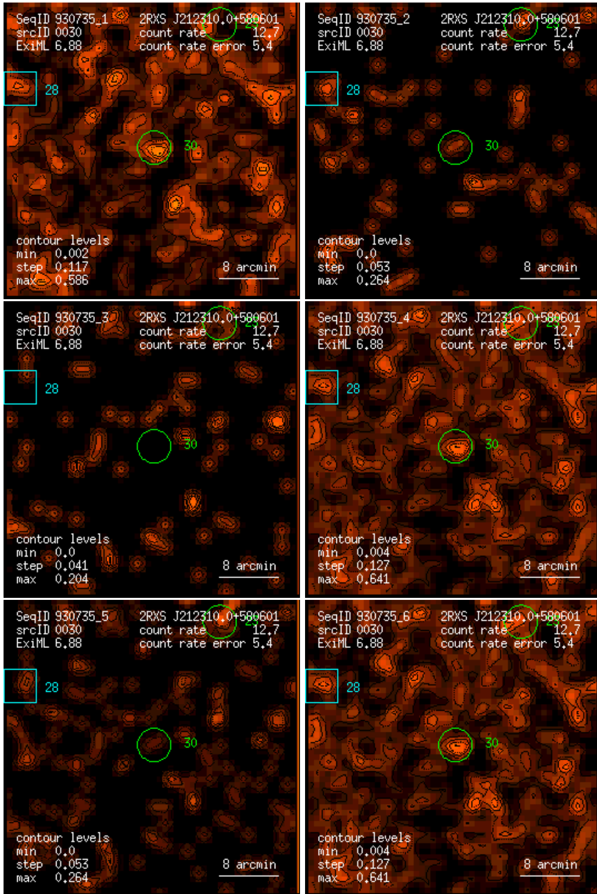
Figure 30: RASS 930735: detection 0030: band rate images, Gaussian filter: (1) PSPC channels 11 – 41, (2) 52 – 90, (3) 91 – 201, (4) 11 – 235, (5) 52 – 201, (6) 11 – 201. Broad band rates in counts/ks. Band rate contour levels in counts/ks/arcmin 2 .
