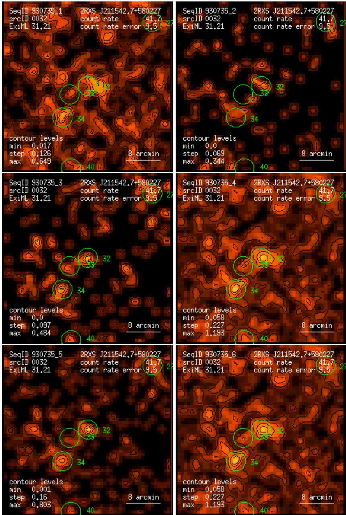
Figure 32: RASS 930735: detection 0032: band rate images, Gaussian filter: (1) PSPC channels 11 – 41, (2) 52 – 90, (3) 91 – 201, (4) 11 – 235, (5) 52 – 201, (6) 11 – 201. Broad band rates in counts/ks. Band rate contour levels in counts/ks/arcmin 2 .
