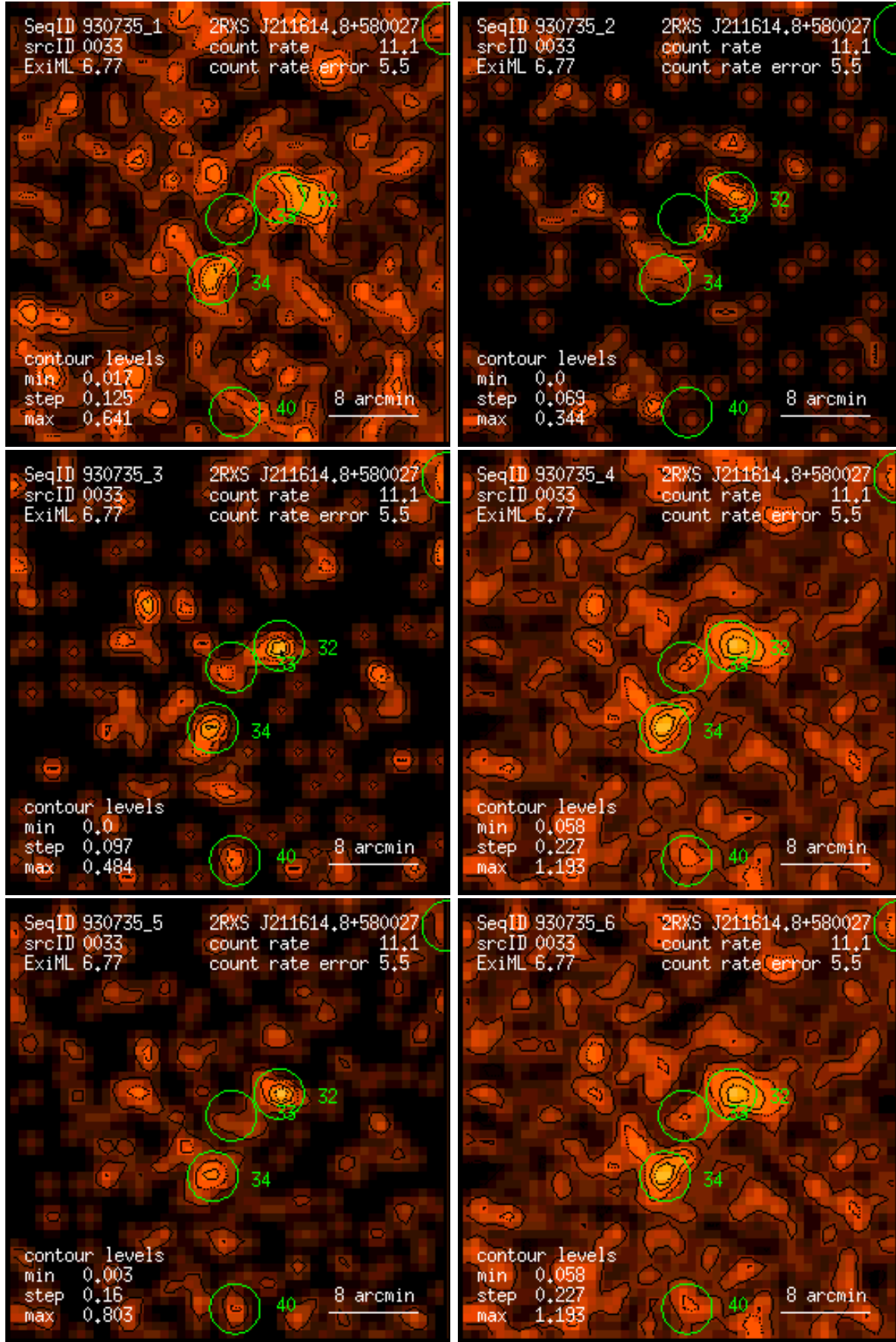
Figure 33: RASS 930735: detection 0033: band rate images, Gaussian filter: (1) PSPC channels 11 – 41, (2) 52 – 90, (3) 91 – 201, (4) 11 – 235, (5) 52 – 201, (6) 11 – 201. Broad band rates in counts/ks. Band rate contour levels in counts/ks/arcmin 2 .
