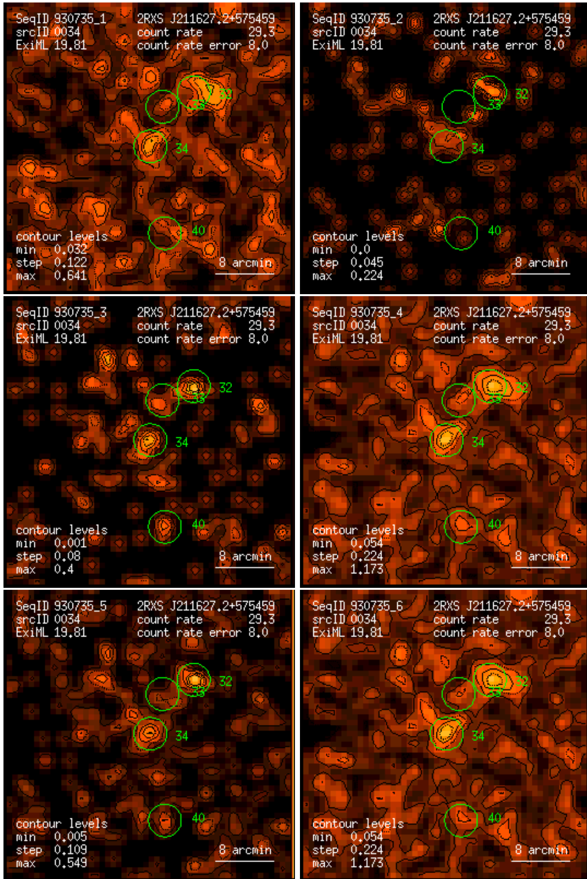
Figure 34: RASS 930735: detection 0034: band rate images, Gaussian filter: (1) PSPC channels 11 – 41, (2) 52 – 90, (3) 91 – 201, (4) 11 – 235, (5) 52 – 201, (6) 11 – 201. Broad band rates in counts/ks. Band rate contour levels in counts/ks/arcmin 2 .
