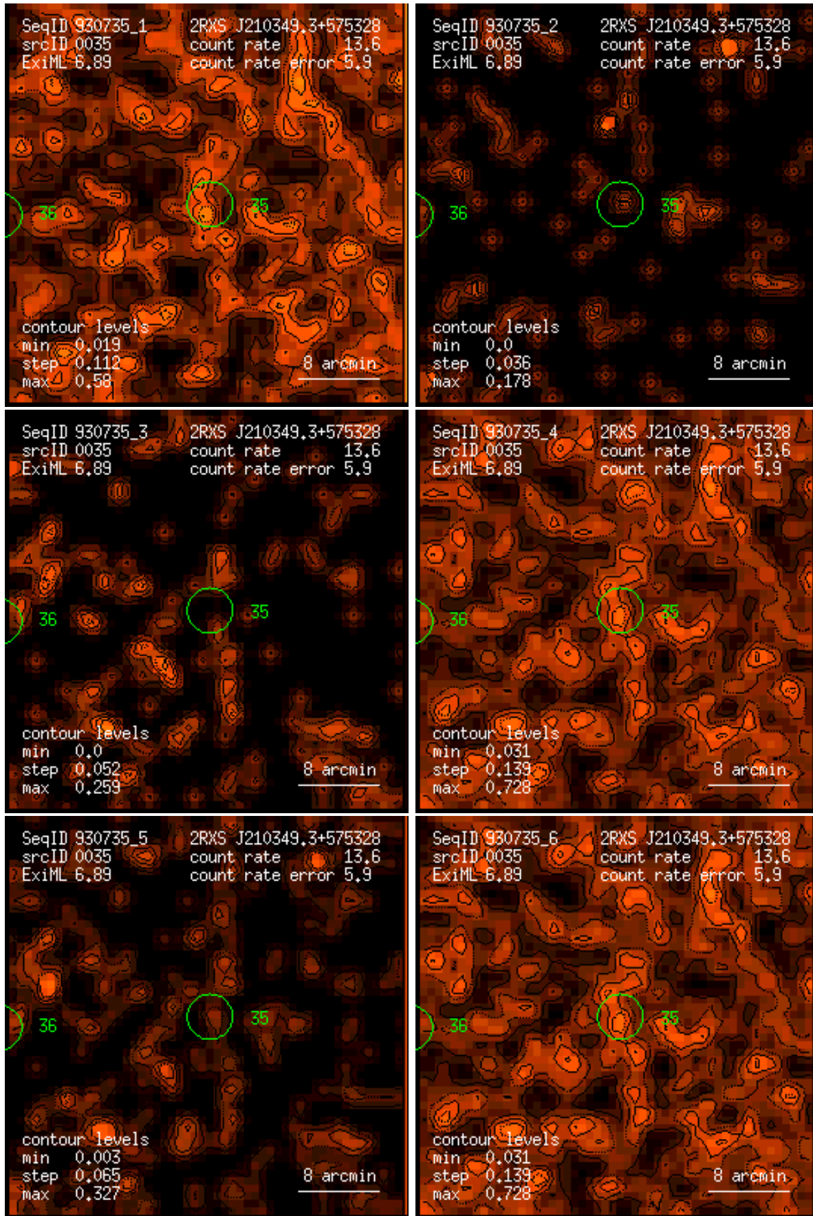
Figure 35: RASS 930735: detection 0035: band rate images, Gaussian filter: (1) PSPC channels 11 – 41, (2) 52 – 90, (3) 91 – 201, (4) 11 – 235, (5) 52 – 201, (6) 11 – 201. Broad band rates in counts/ks. Band rate contour levels in counts/ks/arcmin 2 .
