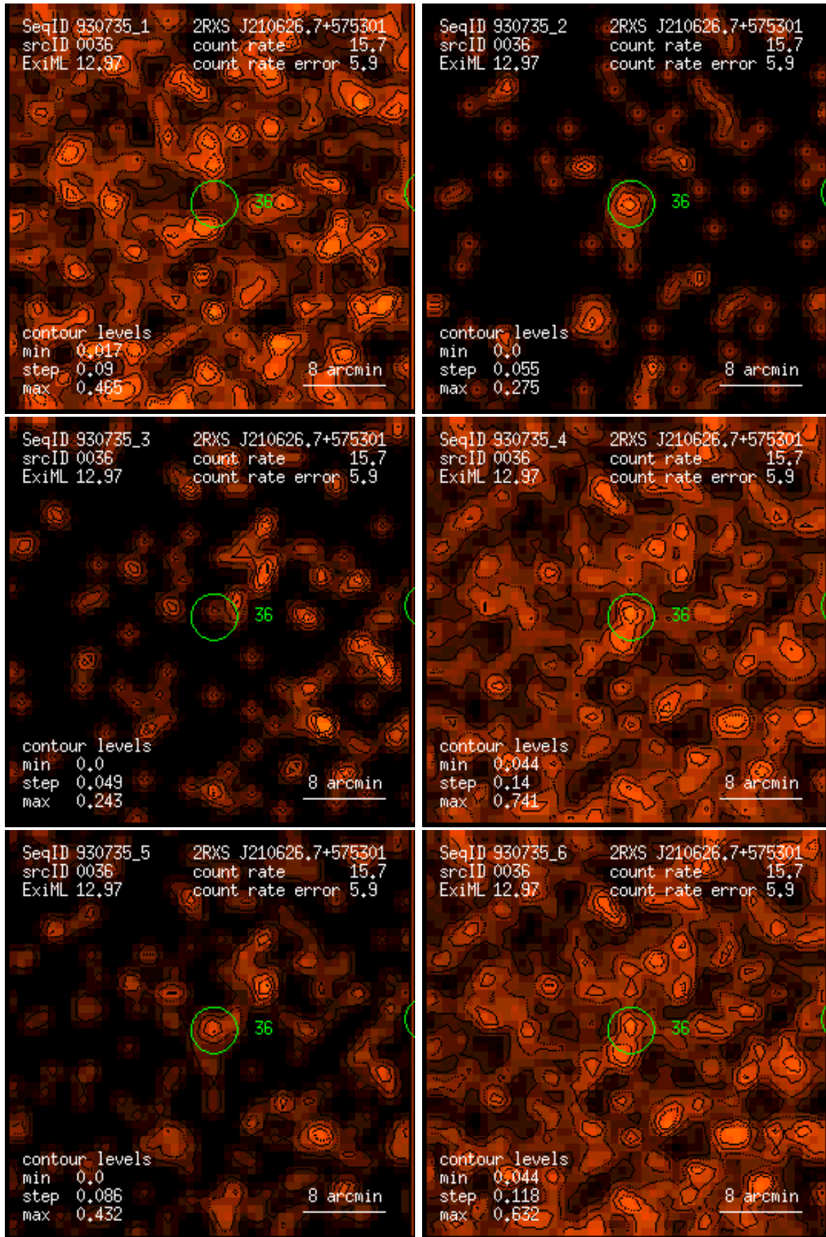
Figure 36: RASS 930735: detection 0036: band rate images, Gaussian filter: (1) PSPC channels 11 – 41, (2) 52 – 90, (3) 91 – 201, (4) 11 – 235, (5) 52 – 201, (6) 11 – 201. Broad band rates in counts/ks. Band rate contour levels in counts/ks/arcmin 2 .
