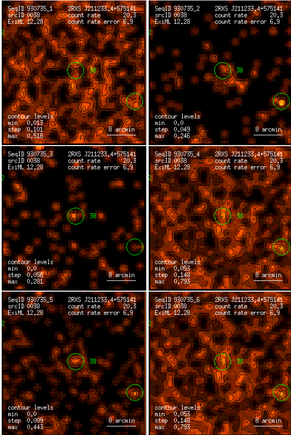
Figure 38: RASS 930735: detection 0038: band rate images, Gaussian filter: (1) PSPC channels 11 – 41, (2) 52 – 90, (3) 91 – 201, (4) 11 – 235, (5) 52 – 201, (6) 11 – 201. Broad band rates in counts/ks. Band rate contour levels in counts/ks/arcmin 2 .
