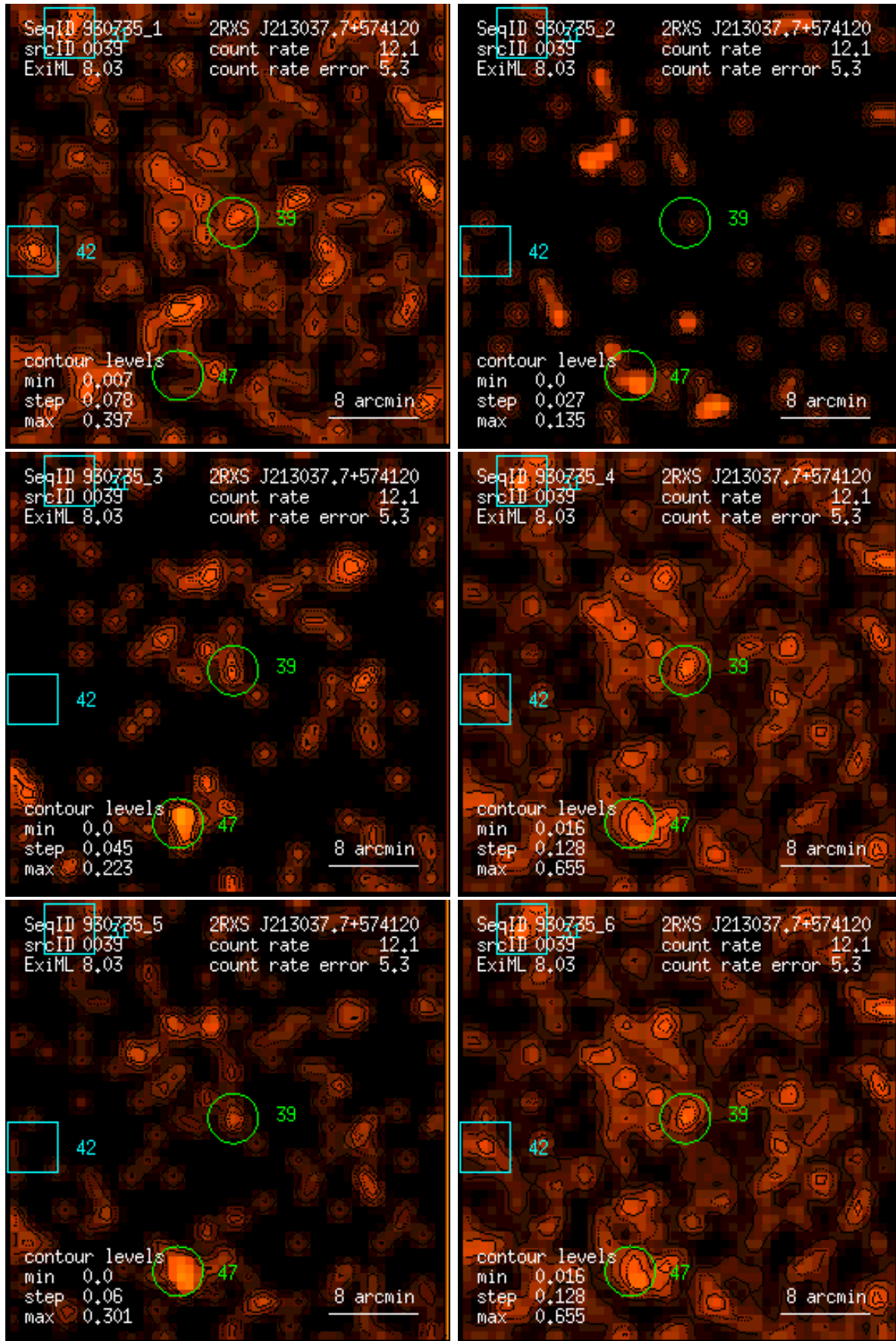
Figure 39: RASS 930735: detection 0039: band rate images, Gaussian filter: (1) PSPC channels 11 – 41, (2) 52 – 90, (3) 91 – 201, (4) 11 – 235, (5) 52 – 201, (6) 11 – 201. Broad band rates in counts/ks. Band rate contour levels in counts/ks/arcmin 2 .
