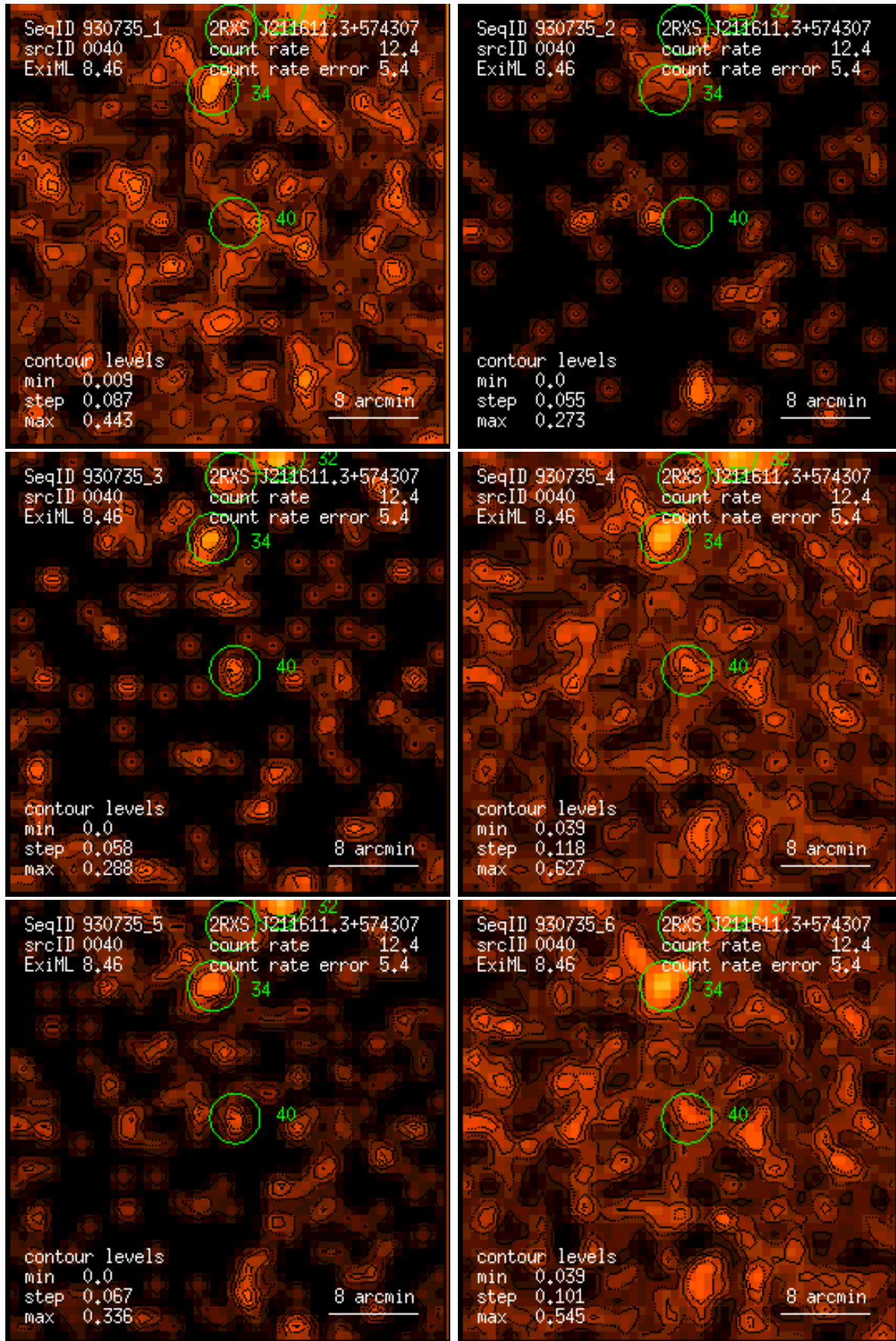
Figure 40: RASS 930735: detection 0040: band rate images, Gaussian filter: (1) PSPC channels 11 – 41, (2) 52 – 90, (3) 91 – 201, (4) 11 – 235, (5) 52 – 201, (6) 11 – 201. Broad band rates in counts/ks. Band rate contour levels in counts/ks/arcmin 2 .
