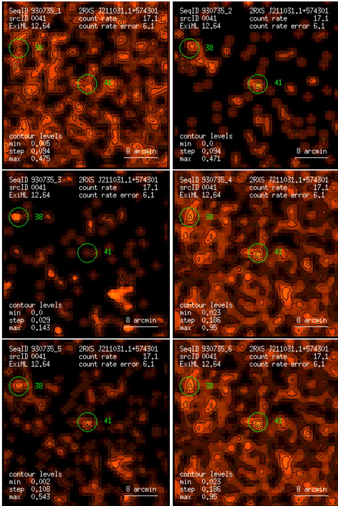
Figure 41: RASS 930735: detection 0041: band rate images, Gaussian filter: (1) PSPC channels 11 – 41, (2) 52 – 90, (3) 91 – 201, (4) 11 – 235, (5) 52 – 201, (6) 11 – 201. Broad band rates in counts/ks. Band rate contour levels in counts/ks/arcmin 2 .
