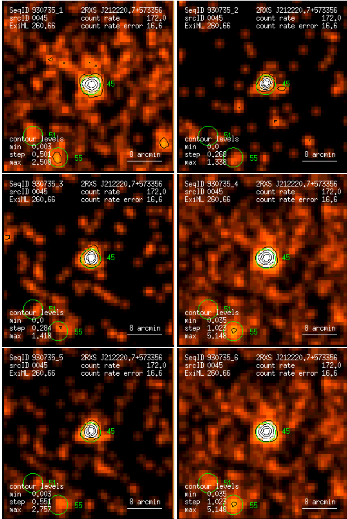
Figure 45: RASS 930735: detection 0045: band rate images, Gaussian filter: (1) PSPC channels 11 – 41, (2) 52 – 90, (3) 91 – 201, (4) 11 – 235, (5) 52 – 201, (6) 11 – 201. Broad band rates in counts/ks. Band rate contour levels in counts/ks/arcmin 2 .
