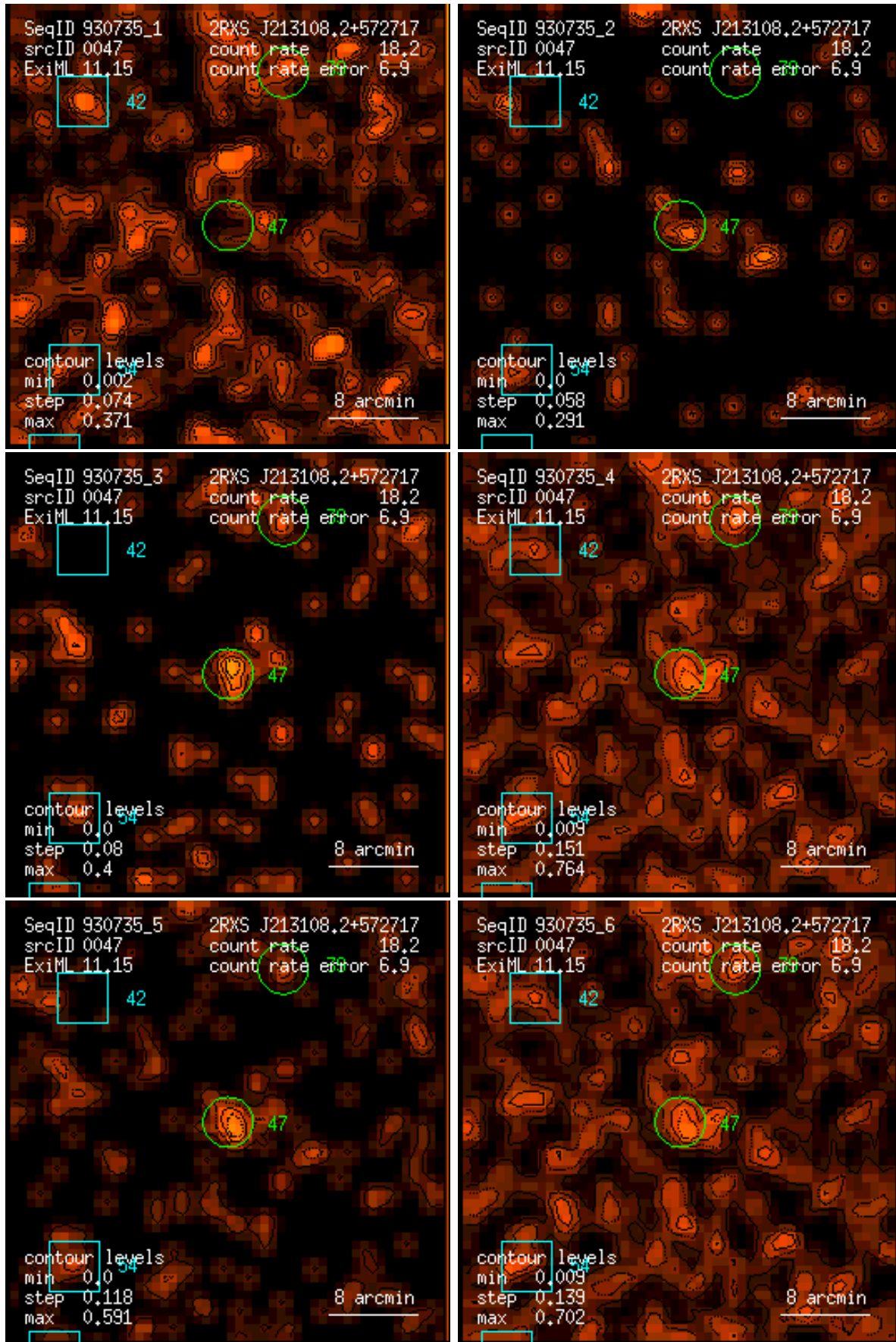
Figure 47: RASS 930735: detection 0047: band rate images, Gaussian filter: (1) PSPC channels 11 – 41, (2) 52 – 90, (3) 91 – 201, (4) 11 – 235, (5) 52 – 201, (6) 11 – 201. Broad band rates in counts/ks. Band rate contour levels in counts/ks/arcmin 2 .
