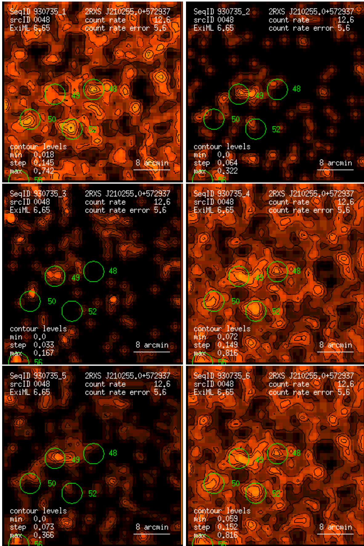
Figure 48: RASS 930735: detection 0048: band rate images, Gaussian filter: (1) PSPC channels 11 – 41, (2) 52 – 90, (3) 91 – 201, (4) 11 – 235, (5) 52 – 201, (6) 11 – 201. Broad band rates in counts/ks. Band rate contour levels in counts/ks/arcmin 2 .
