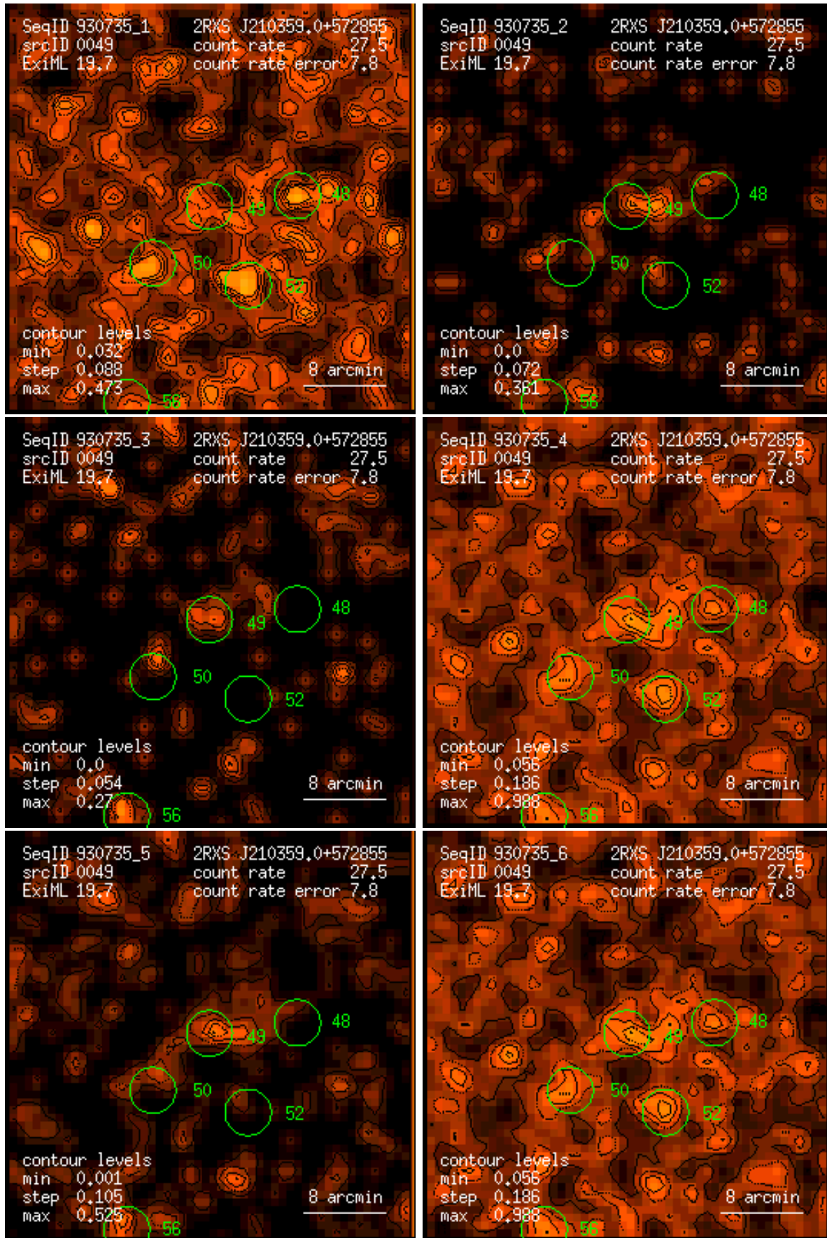
Figure 49: RASS 930735: detection 0049: band rate images, Gaussian filter: (1) PSPC channels 11 – 41, (2) 52 – 90, (3) 91 – 201, (4) 11 – 235, (5) 52 – 201, (6) 11 – 201. Broad band rates in counts/ks. Band rate contour levels in counts/ks/arcmin 2 .
