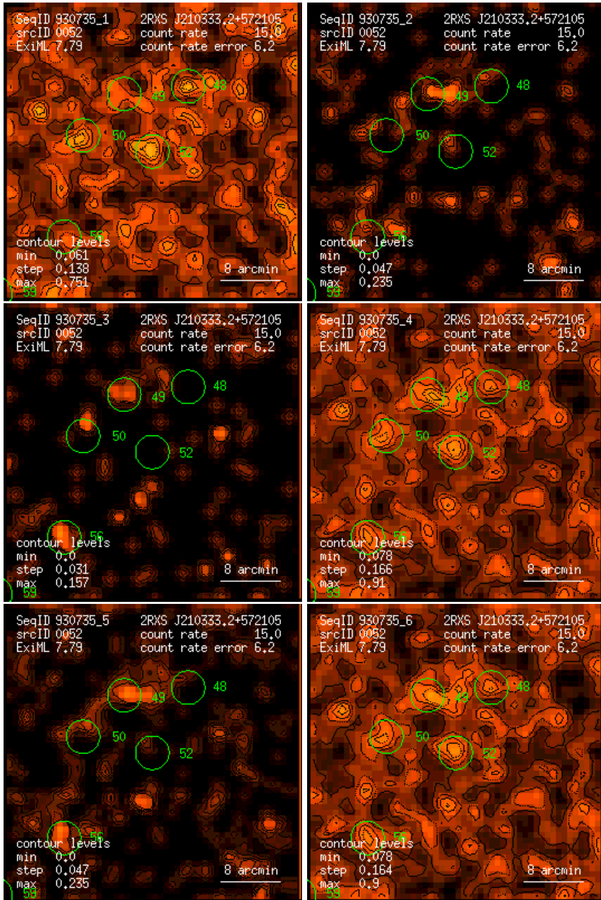
Figure 52: RASS 930735: detection 0052: band rate images, Gaussian filter: (1) PSPC channels 11 – 41, (2) 52 – 90, (3) 91 – 201, (4) 11 – 235, (5) 52 – 201, (6) 11 – 201. Broad band rates in counts/ks. Band rate contour levels in counts/ks/arcmin 2 .
