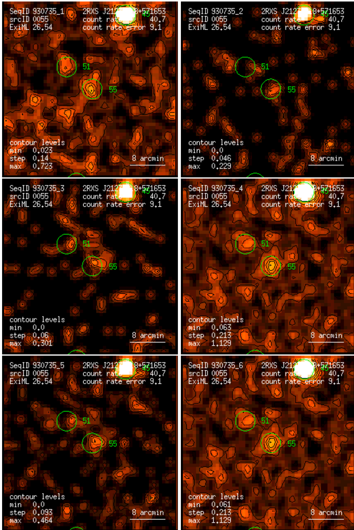
Figure 55: RASS 930735: detection 0055: band rate images, Gaussian filter: (1) PSPC channels 11 – 41, (2) 52 – 90, (3) 91 – 201, (4) 11 – 235, (5) 52 – 201, (6) 11 – 201. Broad band rates in counts/ks. Band rate contour levels in counts/ks/arcmin 2 .
