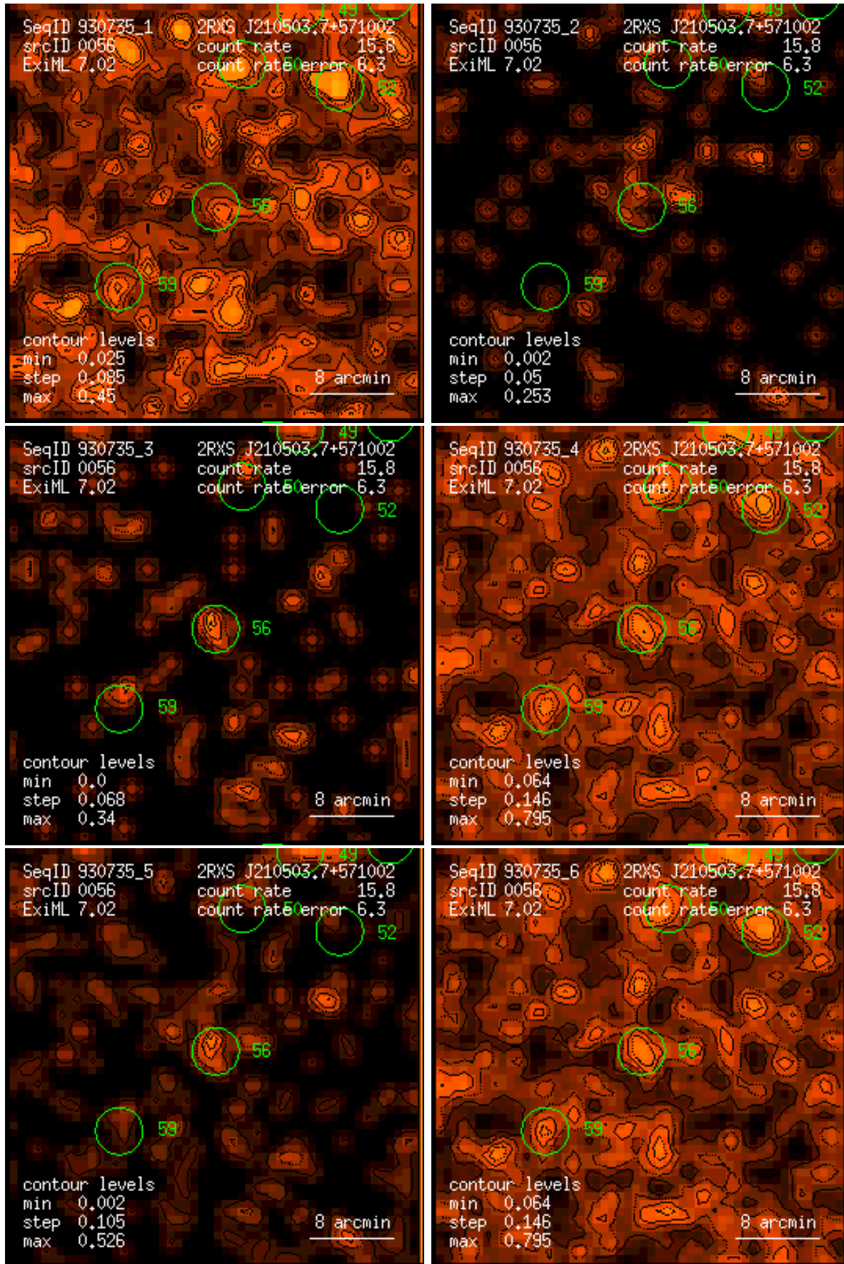
Figure 56: RASS 930735: detection 0056: band rate images, Gaussian filter: (1) PSPC channels 11 – 41, (2) 52 – 90, (3) 91 – 201, (4) 11 – 235, (5) 52 – 201, (6) 11 – 201. Broad band rates in counts/ks. Band rate contour levels in counts/ks/arcmin 2 .
