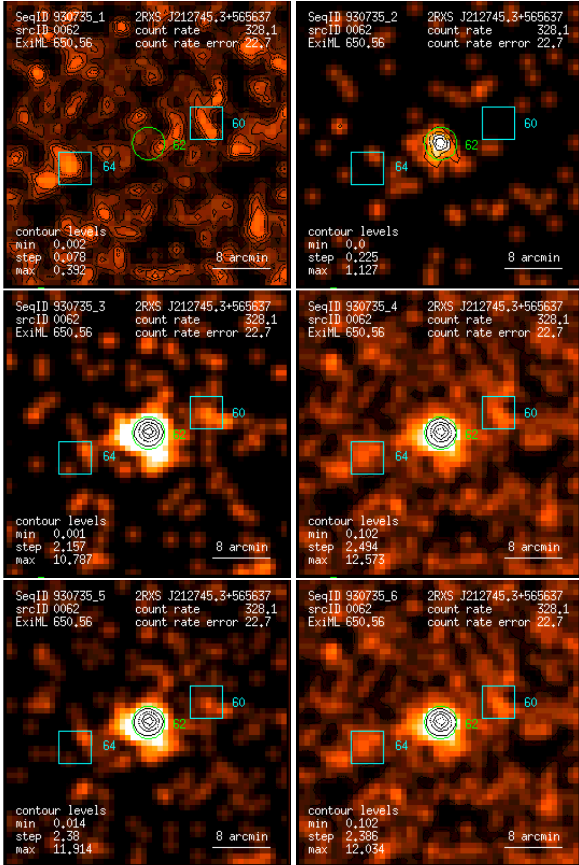
Figure 62: RASS 930735: detection 0062: band rate images, Gaussian filter: (1) PSPC channels 11 – 41, (2) 52 – 90, (3) 91 – 201, (4) 11 – 235, (5) 52 – 201, (6) 11 – 201. Broad band rates in counts/ks. Band rate contour levels in counts/ks/arcmin 2 .
