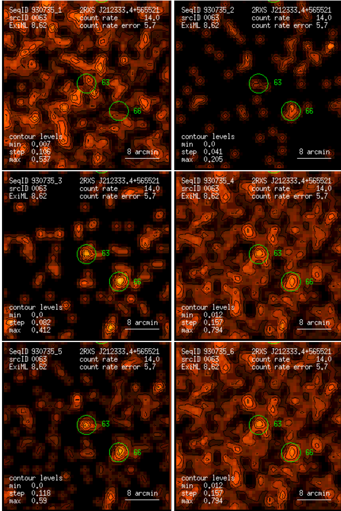
Figure 63: RASS 930735: detection 0063: band rate images, Gaussian filter: (1) PSPC channels 11 – 41, (2) 52 – 90, (3) 91 – 201, (4) 11 – 235, (5) 52 – 201, (6) 11 – 201. Broad band rates in counts/ks. Band rate contour levels in counts/ks/arcmin 2 .
