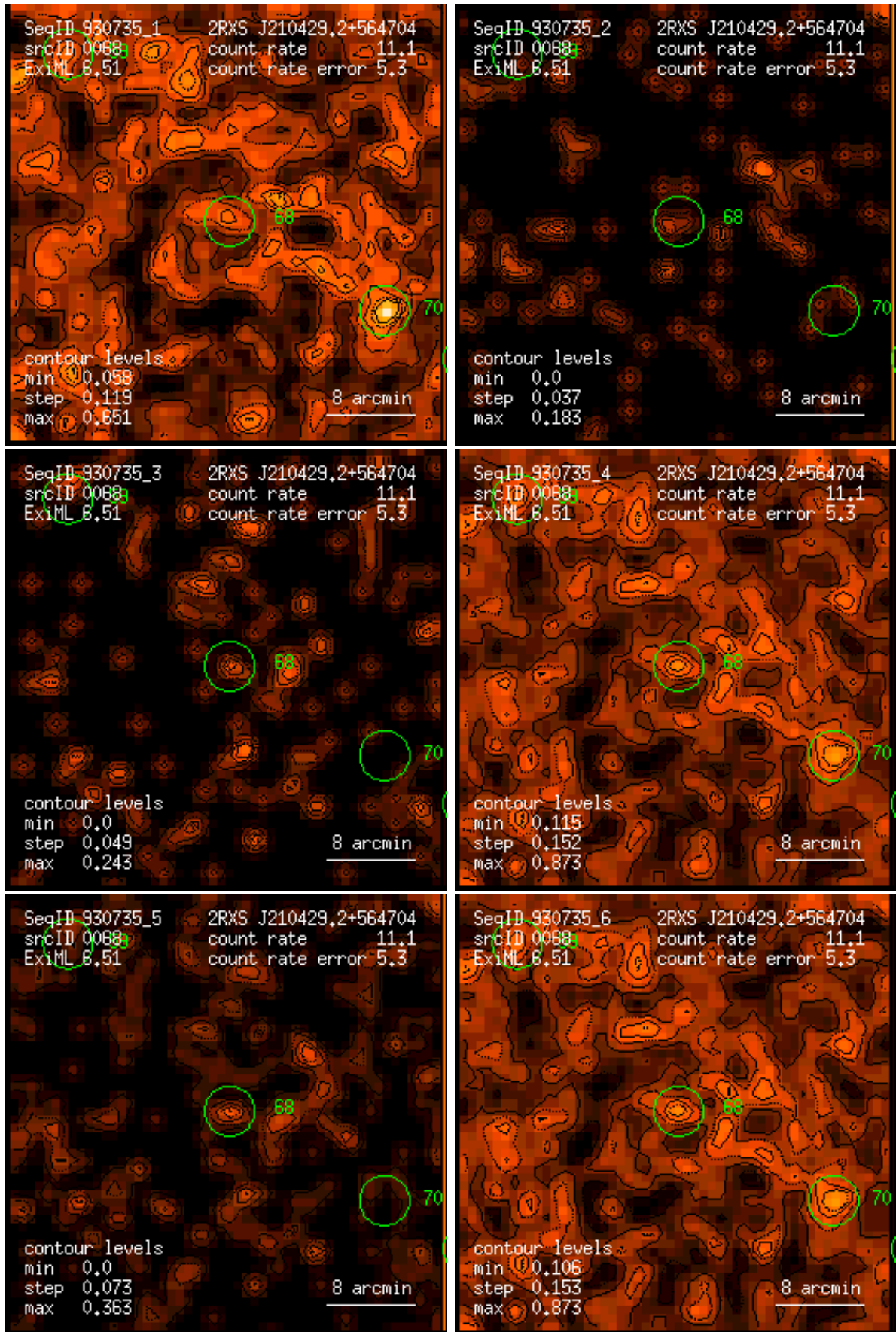
Figure 68: RASS 930735: detection 0068: band rate images, Gaussian filter: (1) PSPC channels 11 – 41, (2) 52 – 90, (3) 91 – 201, (4) 11 – 235, (5) 52 – 201, (6) 11 – 201. Broad band rates in counts/ks. Band rate contour levels in counts/ks/arcmin 2 .
