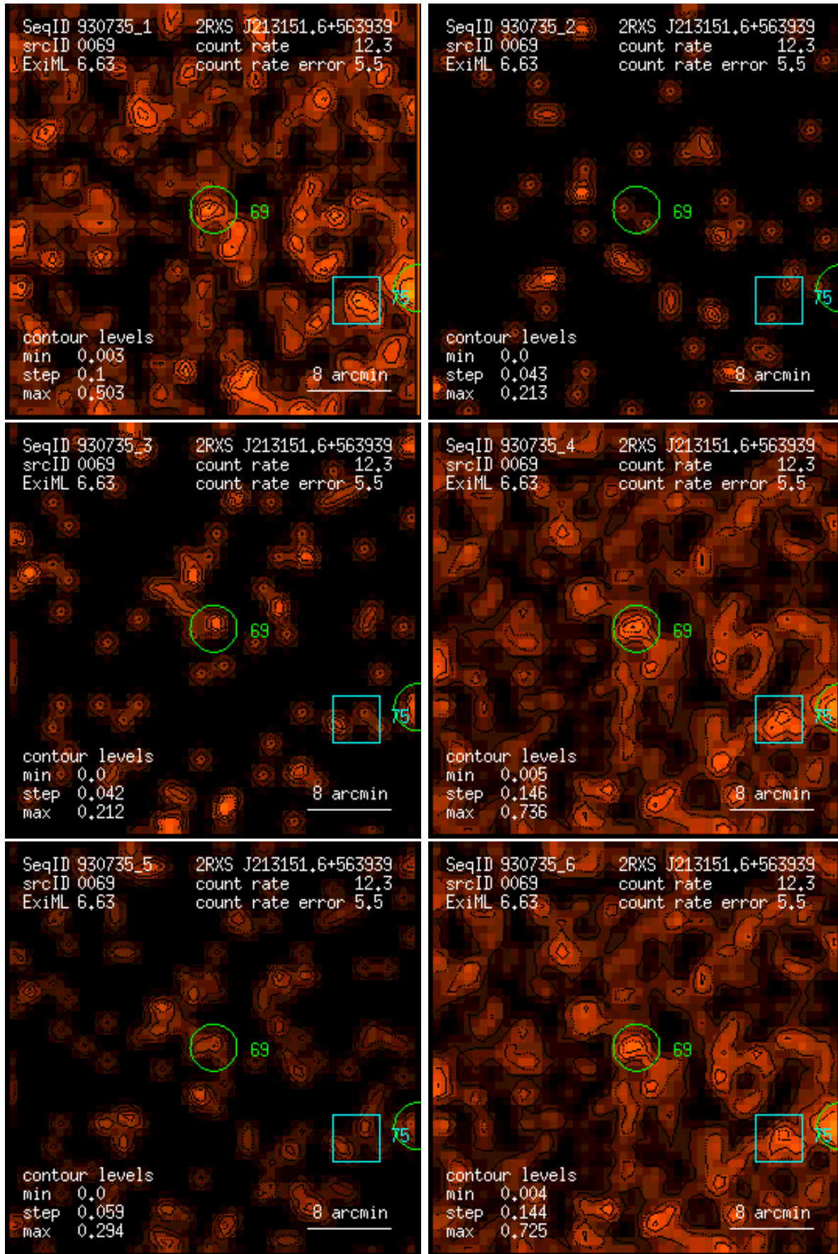
Figure 69: RASS 930735: detection 0069: band rate images, Gaussian filter: (1) PSPC channels 11 – 41, (2) 52 – 90, (3) 91 – 201, (4) 11 – 235, (5) 52 – 201, (6) 11 – 201. Broad band rates in counts/ks. Band rate contour levels in counts/ks/arcmin 2 .
