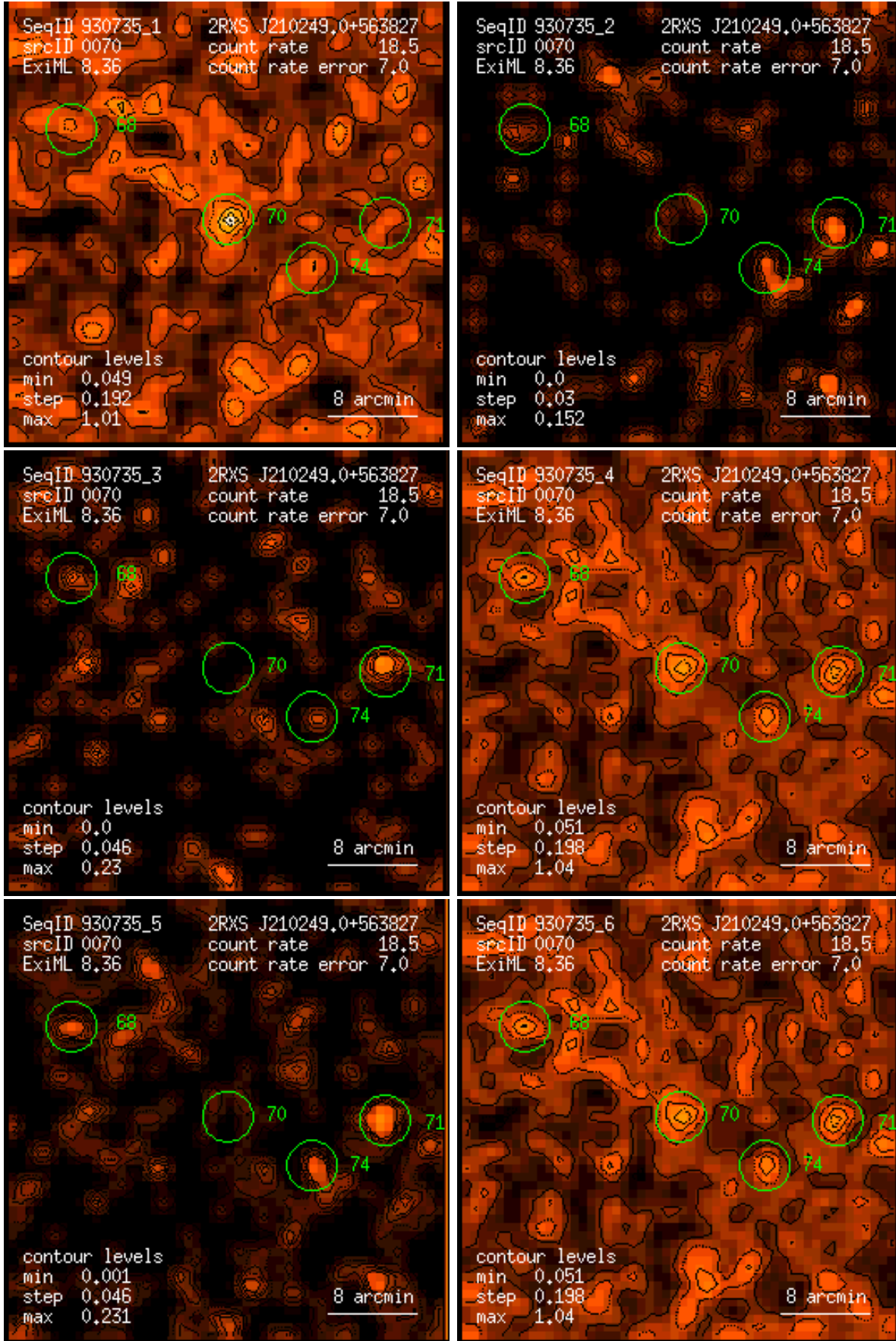
Figure 70: RASS 930735: detection 0070: band rate images, Gaussian filter: (1) PSPC channels 11 – 41, (2) 52 – 90, (3) 91 – 201, (4) 11 – 235, (5) 52 – 201, (6) 11 – 201. Broad band rates in counts/ks. Band rate contour levels in counts/ks/arcmin 2 .
